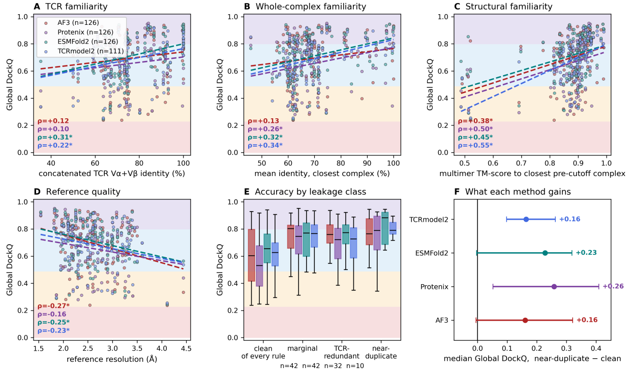
Figure 5: What accuracy tracks besides the model. (A) Global DockQ against concatenated TCR V \alpha +V \beta identity to the closest pre-cutoff complex, (B) against mean identity across all chains of the closest complex, (C) against the multimer TM-score between the target’s own experimental structure and the closest pre-cutoff complex, and (D) against the resolution of the experimental reference; dashed lines are per-method linear fits and \rho is Spearman, starred where p < 0.05 . (E) Accuracy by audit class. (F) Median Global DockQ gained on the 10 near-duplicates relative to the 42 targets clean of every criterion, with 95% bootstrap intervals. Shaded bands in A–E are the CAPRI quality classes.
