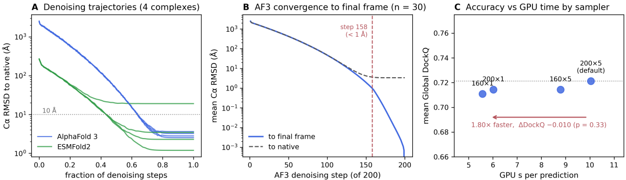
Figure 6: Denoising trajectories and AlphaFold 3 sampler economy. (A) C\alpha RMSD to the native along the denoising trajectory for four complexes traced in both models; AlphaFold 3 (200 steps, initial \sigma \approx 2,560 Å) is still tens of ångströms out at its midpoint, ESMFold2 (68 recorded steps, initial \sigma \approx 256 Å) is within a few ångströms. (B) AlphaFold 3 convergence to its own final frame over 30 complexes \times 5 samples; band spans median to 90th percentile. (C) GPU time against mean Global DockQ for four sampler configurations on the same 30 complexes.
