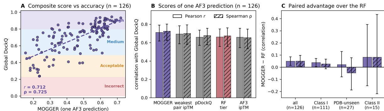
Figure 4: A composite single-prediction score against the published alternatives. (A) Global DockQ against MOGGER for the 126 complexes, with the linear fit and both correlations; shaded bands are the CAPRI quality classes. (B) Correlation with Global DockQ for every score computable from one AlphaFold 3 prediction, over all 126 complexes; whiskers are 95% bootstrap intervals. (C) Paired MOGGER-minus random-forest difference in each correlation, by subset; whiskers are 95% paired-bootstrap intervals, and only the full benchmark excludes zero.
