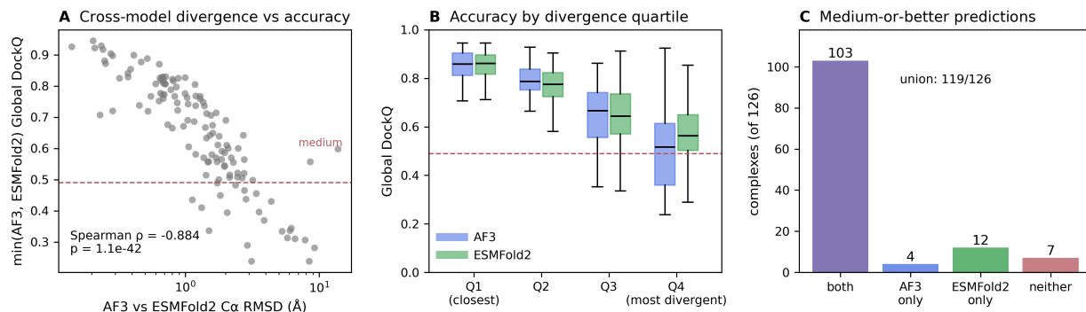
Figure 6: Structural divergence between the AlphaFold 3 and ESMFold2 predictions. (A) Cα RMSD between the AlphaFold 3 and ESMFold2 predictions of the same sequence against the worse of their two Global DockQ scores. (B) Global DockQ by quartile of that divergence; the two methods degrade together. (C) Complexes reaching medium-or-better accuracy: individually, jointly, and neither.
