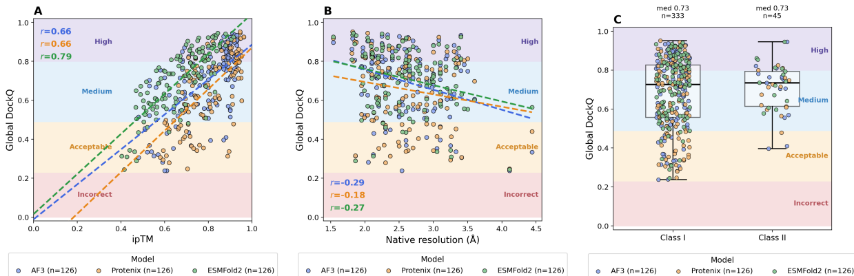
Figure 4: Determinants of interface accuracy. (A) Global DockQ against each method’s own ipTM, with per-method linear fits and Pearson r . ESMFold2’s confidence is both more conservative — it reaches a given DockQ at a lower ipTM — and better ordered. (B) Global DockQ against the resolution of the experimental reference. (C) Global DockQ by MHC class. Shaded bands are the CAPRI quality classes.
