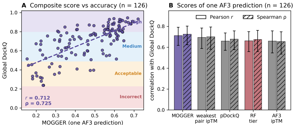
Figure 5: A composite single-prediction score against the published alternatives. (A) Global DockQ against MOGGER for the 126 complexes, with the linear fit and both correlations; shaded bands are the CAPRI quality classes. (B) Correlation with Global DockQ for every score computable from one AlphaFold 3 prediction, over all 126 complexes; whiskers are 95% bootstrap intervals.
