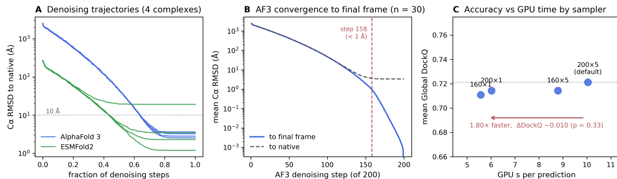
Figure 7: Denoising trajectories and AlphaFold 3 sampler economy. (A) C\alpha RMSD to the native along the denoising trajectory for four complexes traced in both models; AlphaFold 3 (200 steps, initial \sigma \approx 2,560 Å) is still tens of ångströms out at its midpoint, ESMFold2 (68 recorded steps, initial \sigma \approx 256 Å) is within a few ångströms. (B) AlphaFold 3 convergence to its own final frame over 30 complexes \times 5 samples; band spans median to 90th percentile. (C) GPU time against mean Global DockQ for four sampler configurations on the same 30 complexes.
