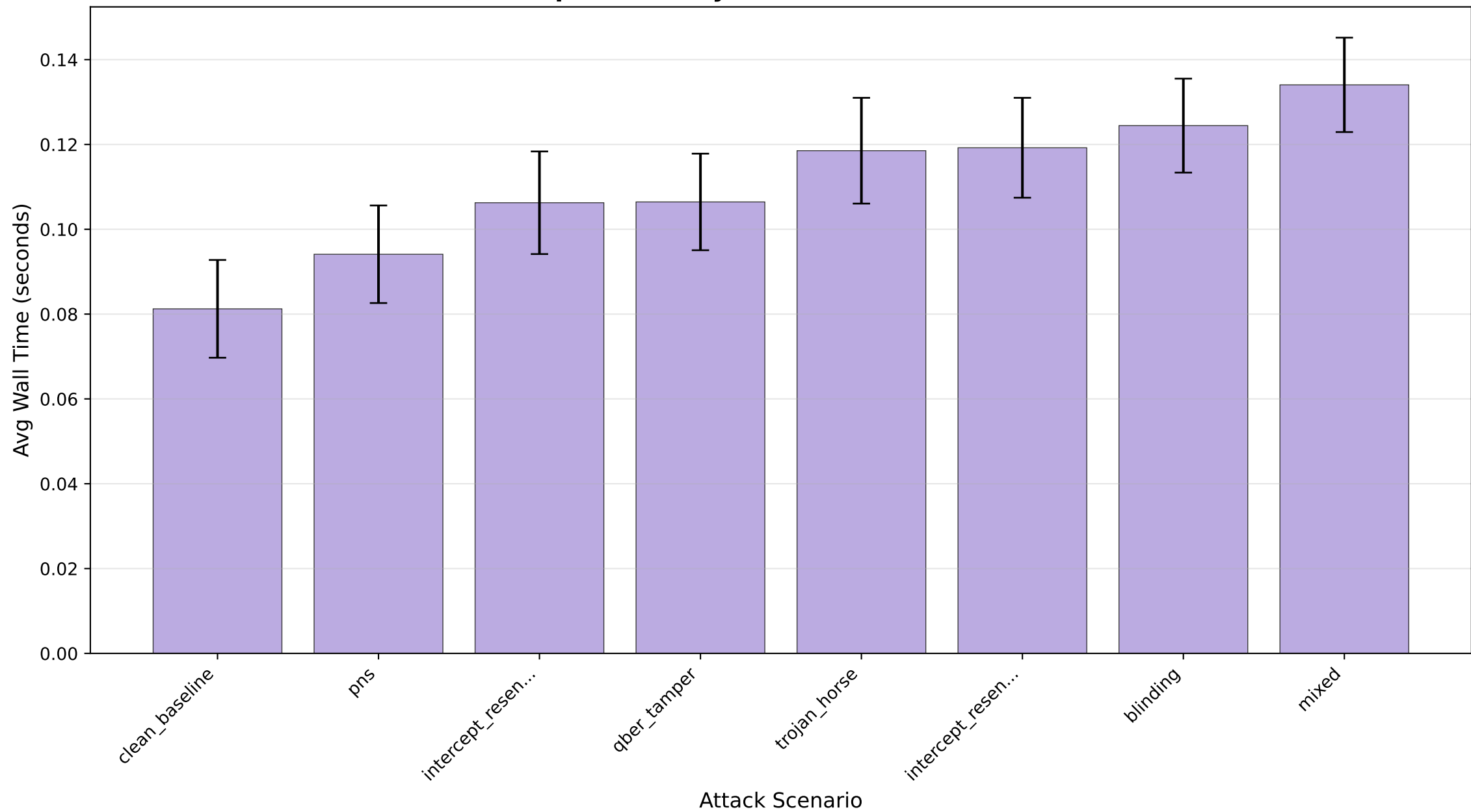
RQ5 - Reproducibility: Execution Time Distribution
