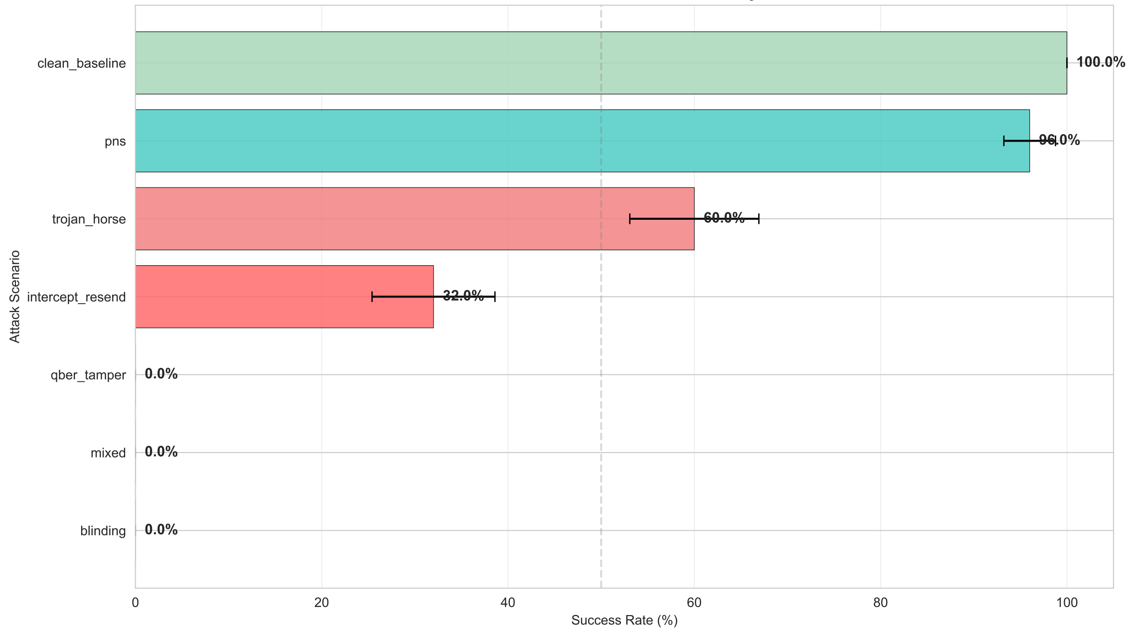
RQ1 - Attack Effectiveness: Success Rate by Scenario
