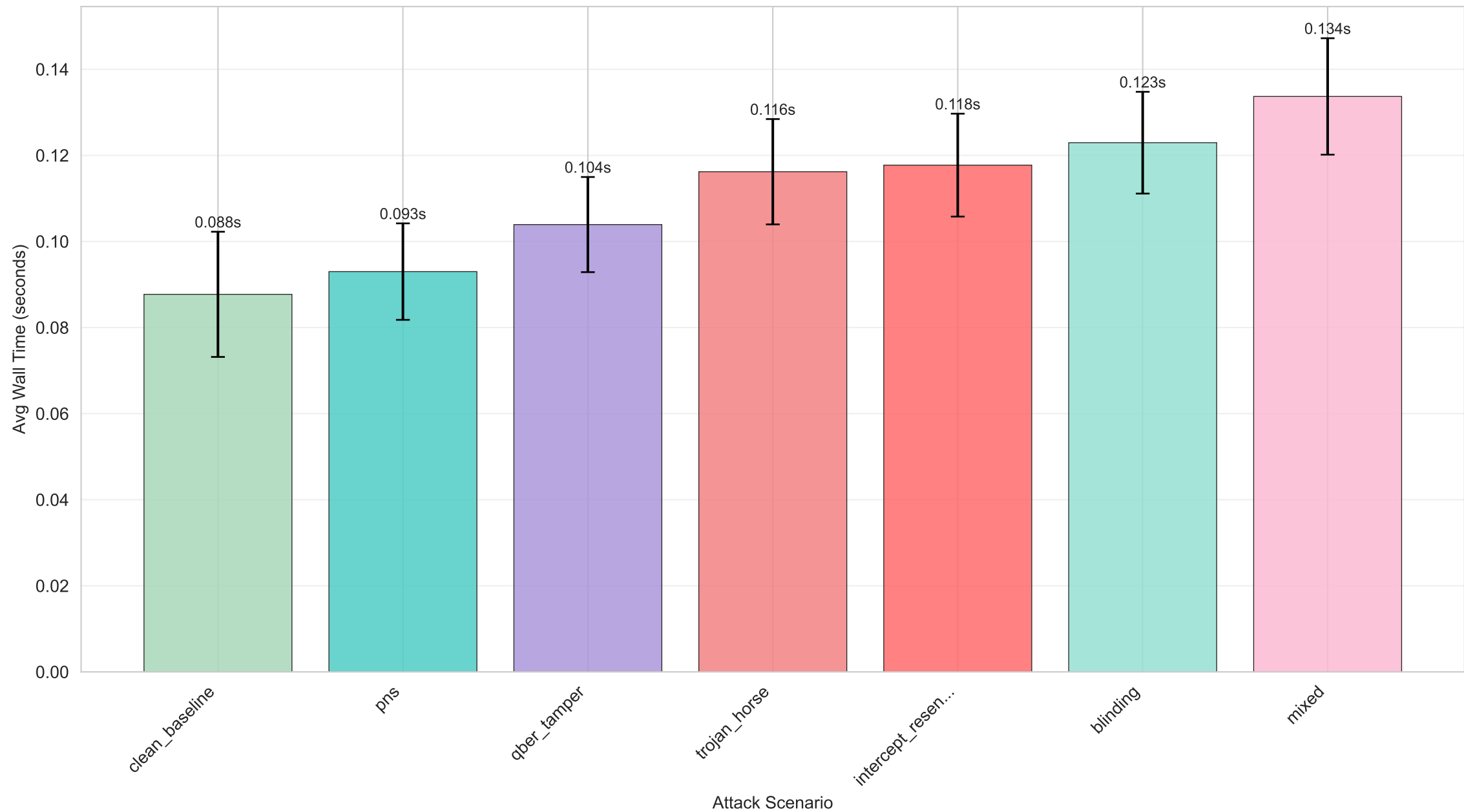
RQ5 - Robustness: Execution Time Distribution
