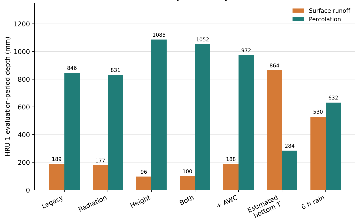
B HRU 1: interface and boundary sensitivity
