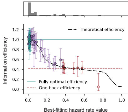
Information efficiency vs best-fitting hazard rate
