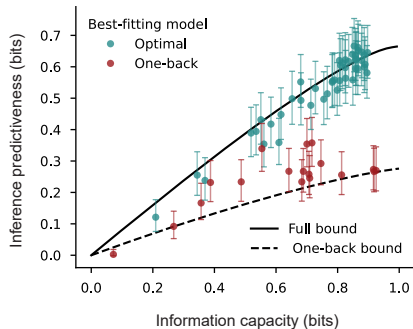
Optimal vs heuristic model comparison Bead-prediction experiment
