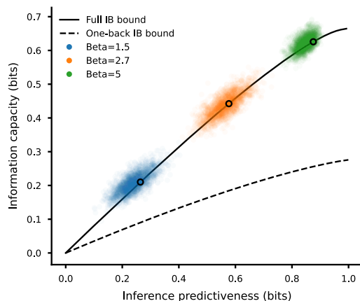
Bead prediction task Single trial set (500 bead draws) 2000 choice set samples (fully optimal model) Error from choice sampling
