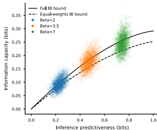
Horse prediction, intermediate W-S ratio (2.5:1) Single trial set (600 horse races) 2000 choice set samples (fully optimal model) Error from choice sampling + trial set sampling
