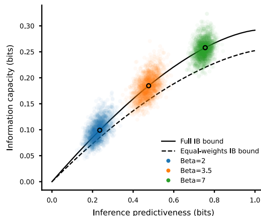
Horse prediction, intermediate W-S ratio (2.5:1) Single trial set (600 horse races) 2000 choice set samples (fully optimal model) Error from choice sampling
