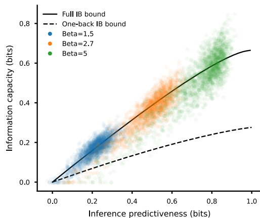
Bead prediction task 2000 different trial sets (500 bead draws) 1 choice set sample per trial set (fully optimal model) Error from choice sampling + trial set sampling
