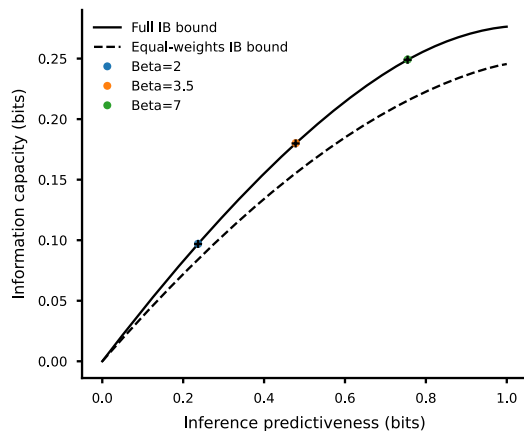
Horse prediction, intermediate W-S ratio (2.5:1) Single trial set (10000000 horse races) 20 choice set samples (fully optimal model) No estimator
