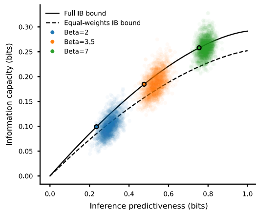
Horse prediction, intermediate W-S ratio (2.5:1) Single trial set (600 horse races) 2000 choice set samples (fully optimal model) No estimator
