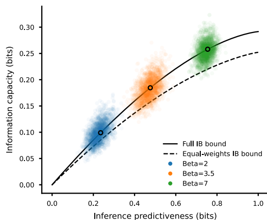
Horse prediction, intermediate W-S ratio (2.5:1) Single trial set (600 horse races) 2000 choice set samples (fully optimal model) NSB estimator
