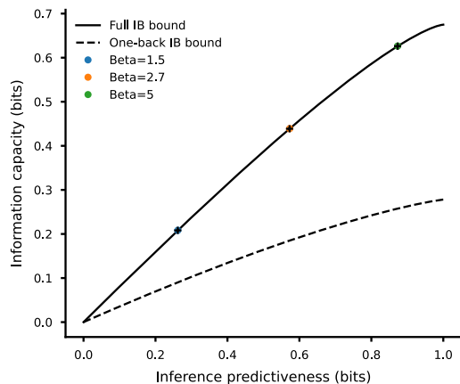
Bead prediction task Single large N trial set (10000000 bead draws) 20 choice set samples (fully optimal model) No estimator
