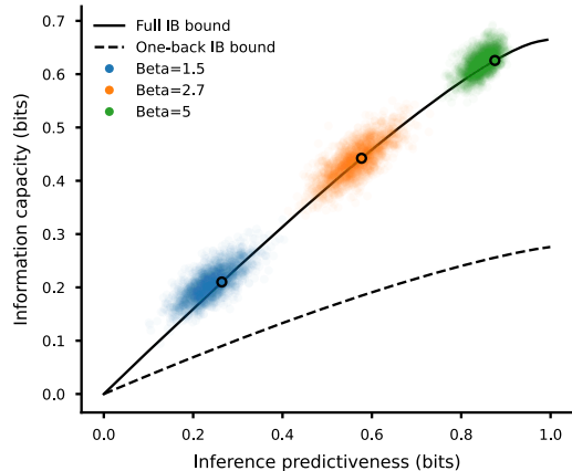
Bead prediction task Single trial set (500 bead draws) 2000 choice set samples (fully optimal model) NSB estimator
