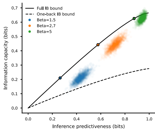
Bead prediction task Single trial set (500 bead draws) 2000 choice set samples (fully optimal model) No estimator
