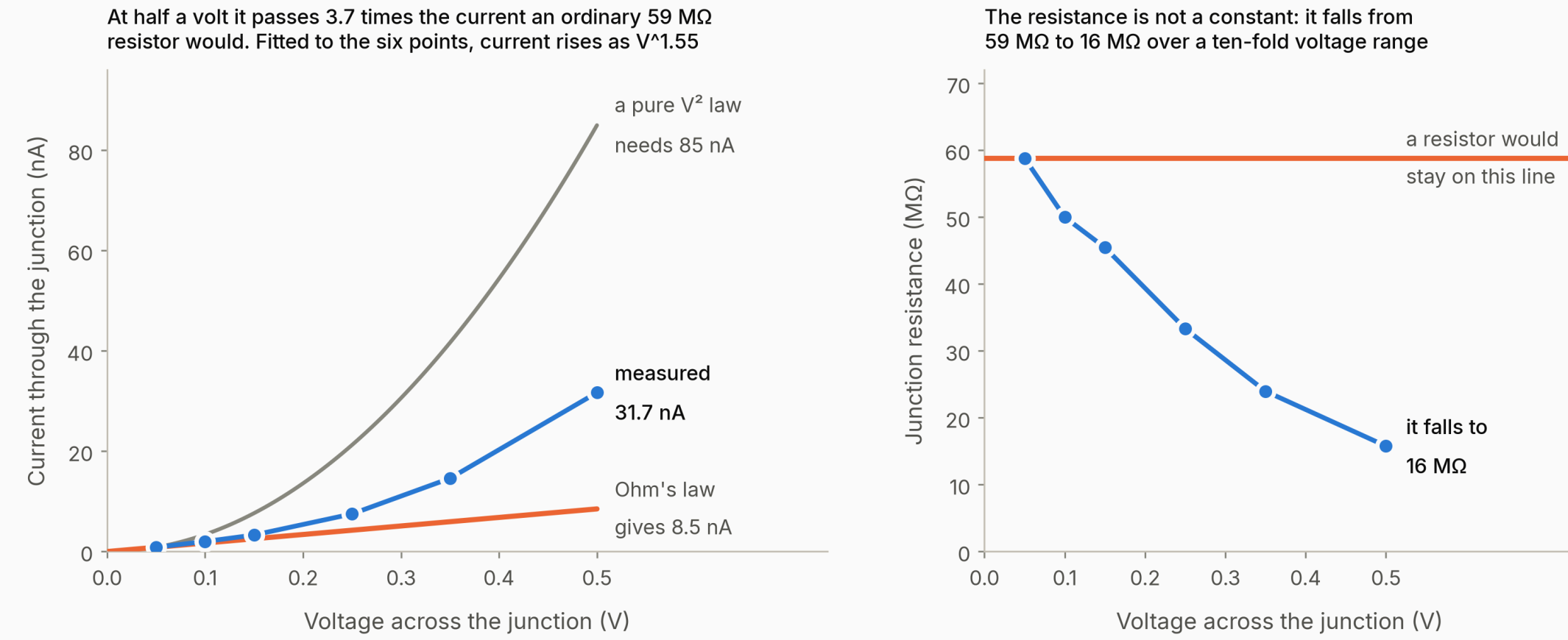
Current rose from 0.85 nA at 0.05 V to 31.7 nA at 0.5 V — 3.7 times faster than Ohm's law , fitting V^{1.55} , with the junction resistance falling from 59 to 16 MΩ. Eight rounds with the polarities interleaved, so drift could not manufacture a slope: symmetric both ways to about 10%, confirmed by a bias-rip test on two separate nights. That rules out a metallic short, which would be ohmic, and an open circuit, which would give nothing. Source: sessions/2026-09-17-bench.md §3.15.
