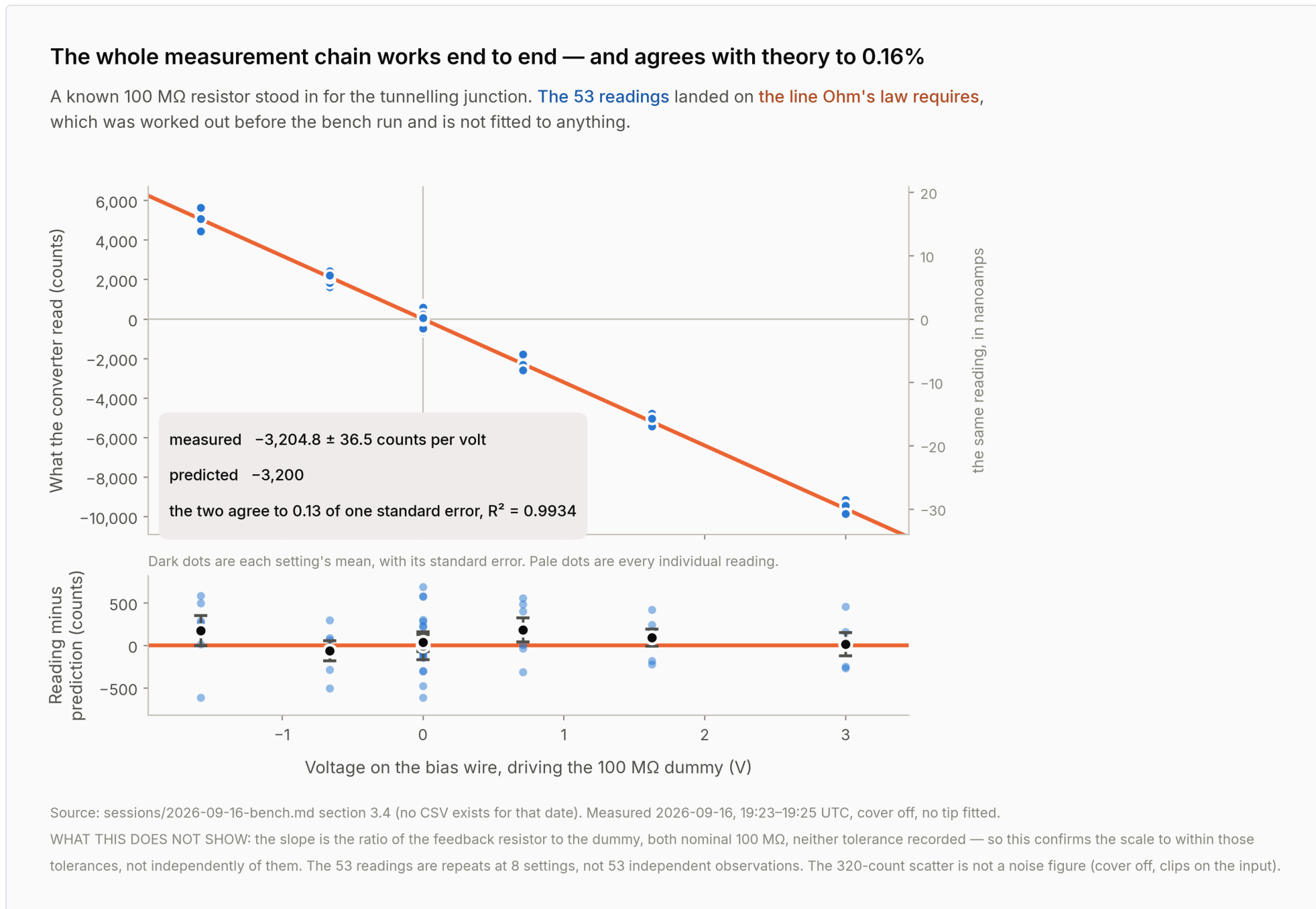
Measured \sim 3,204.8 \pm 36.5 counts per volt against \sim 3,200 predicted — agreement to 0.13 of one standard error, R^2 = 0.9934 over 53 readings. Twelve stages had to be right at once for those points to land on that line. Source: sessions/2026-09-16-bench.md §3.4. What it does not show: the slope is the ratio of two nominally 100 M \Omega resistors whose tolerances were never recorded, and the 53 readings are repeats at 8 settings, not 53 independent observations.
