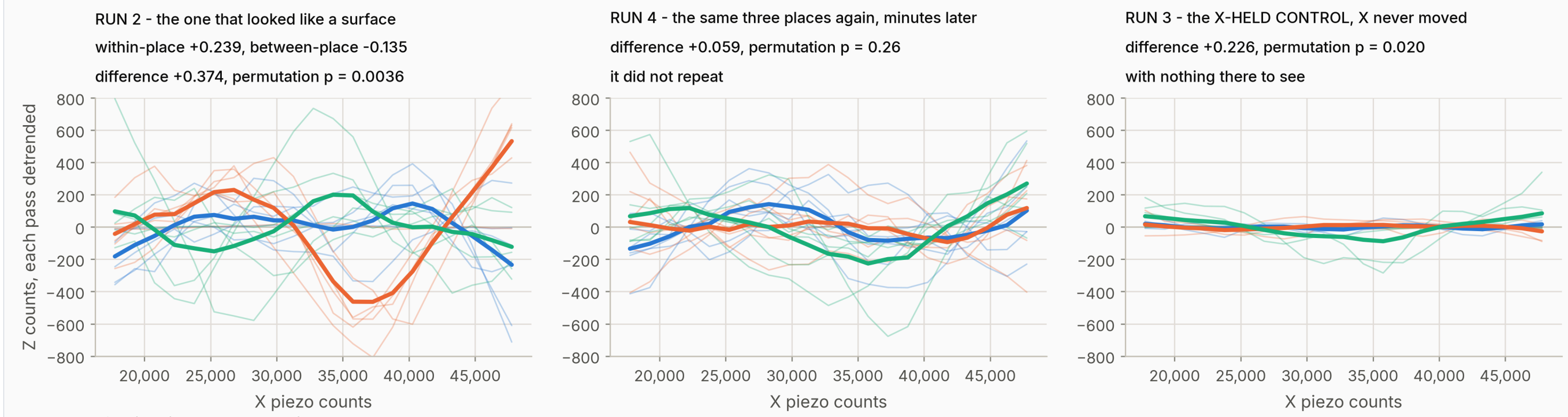
Source: sessions/data/2026-09-19-bench/ycntrl_run2_ypsp12000.csv, ycntrl_run4_ypsp12000_repeat.csv, ycntrl_run3_ypsp12000_xheld.csv. Measured 2026-09-19 between 03:48 and 03:53 UTC; sessions/2026-09-19-bench.md §3.15. Each pass detrended in X, the project's own convention (Code/pc1stm_y_control.py). Every file is 3 places x 6 passes x 21 points - no truncation. THE STATISTICS ARE PERMUTATION TESTS, not the 3.9 sigma reported on the night: that sigma treated overlapping pairs as independent, and was withdrawn at the 2026-09-19 pause point (candidates/VERDICT.md 4). WHAT THIS DOES NOT SHOW: It is not an image and it is not evidence of one. Across 209 reproducibility tests on this data the honest threshold is p < 2.4e-4 - run 2 falls a factor of 14 short of it. Neither log carries a timestamp, so the interval between runs is UNKNOWN, bounded by the \sim 5 minutes between the sections around them (LEAD_VERIFICATION.md V9). Axes are in DAC counts: this instrument has never established a distance scale. The one measurement that still looks like a surface. Six passes at each of three places: passes at the same place agreed +0.239 while different places disagreed -0.135 . The repeat, minutes later, gave +0.056 — and an X-held control, which cannot contain a surface, scored p = 0.020 on the same statistic. Against 209 reproducibility tests the honest threshold is p < 2.4 \times 10^{-4} . Not an image, and not presented as one.
