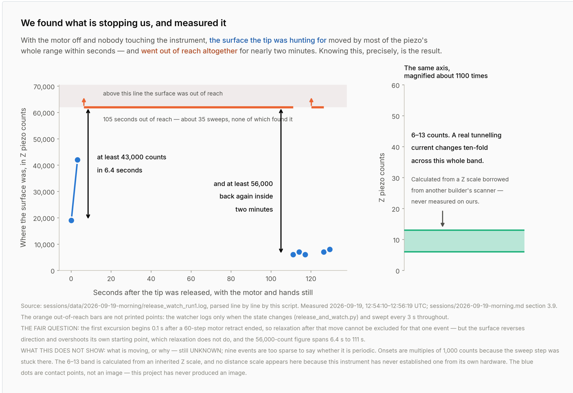
The surface moved by more than 43,000 Z counts within 6.4 seconds, and by more than 56,000 within two minutes — most of the piezo's whole range — and went out of reach altogether for 105 seconds. Source: sessions/data/2026-09-19-morning/release_watch_run1.log. The fair question: the fast excursion begins 0.1 s after a motor retract ended, so relaxation cannot be excluded for that one event — but the motion reverses and overshoots its own starting point, which relaxation does not do, and the two-minute figure is measured long after any transient.
