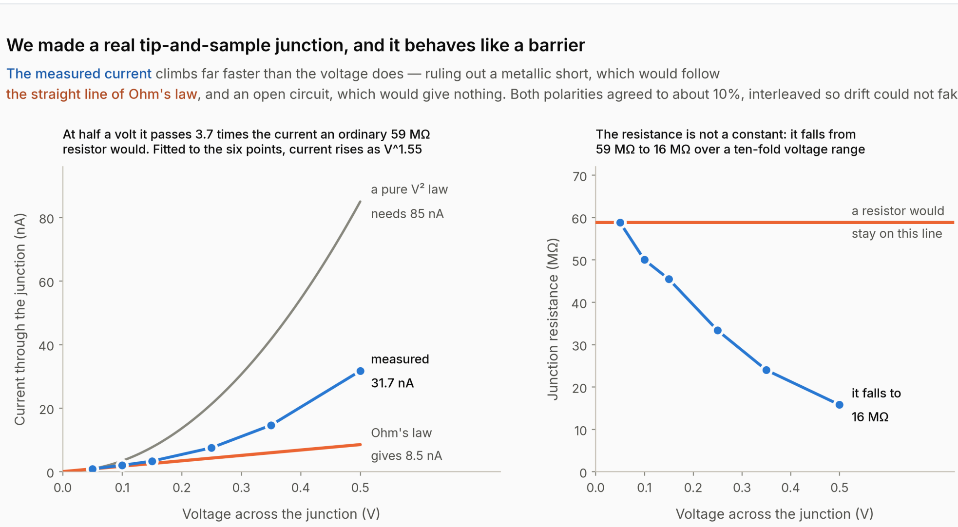
Source: sessions/2026-09-17-bench.md section 3.15, round 7 of 8 (no CSV exists for this sweep). Measured 2026-09-17 from about 19:54:51 UTC, on the 2026-09-17 tip and sample. WHAT THIS SHOWS AND WHAT IT DOES NOT: A barrier conducting at these resistances is conducting by tunnelling, and that much is a claim this figure supports. What it does NOT show is a vacuum tunnelling gap — a contaminant film, a thin oxide or a dirty near-contact are all superlinear too, and tunnelling through a pressed film is still tunnelling but is not a gap you can command, sweep and image with. 16–59 MΩ sits at the low end of the range tunnelling occupies, which usually starts above 100 MΩ. A different tip and sample two nights later gave a different verdict (figure §3). The session log's 'roughly V 1/5 ' reading is wrong; the refit is V 1/5.5 .
