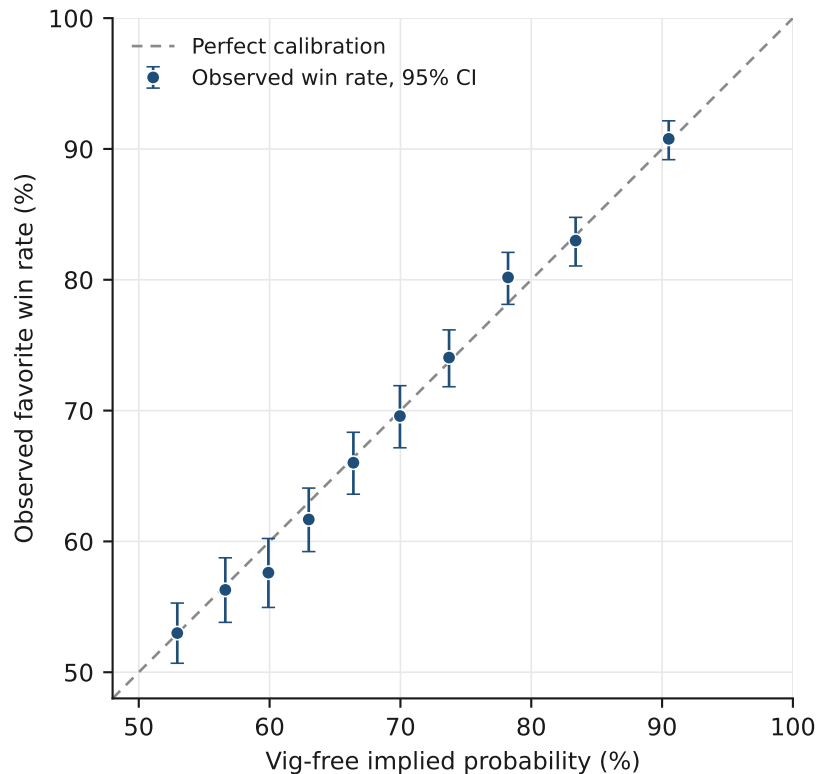
Figure 1. Calibration by decile of implied probability
