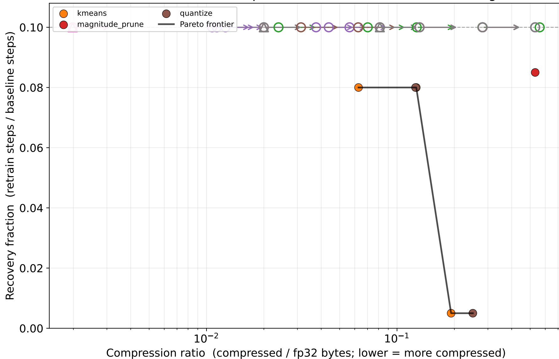
Weight-compression recovery: compression vs. retraining cost ResNet-20 / CIFAR-10 (open markers = DNR within 10% budget)
