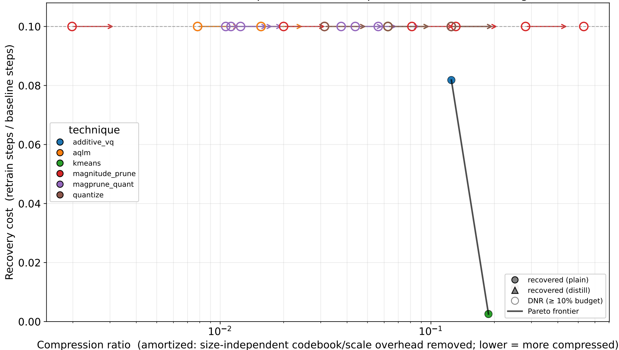
Weight-compression recovery: compression vs. retraining cost ResNet-20 / CIFAR-10 (open markers at top = DNR within 10% budget)
