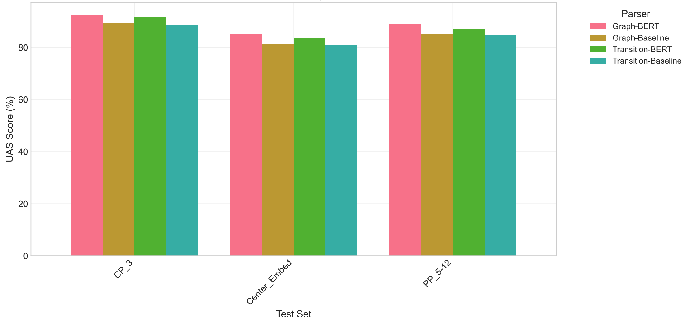
UAS Performance by Test Set
