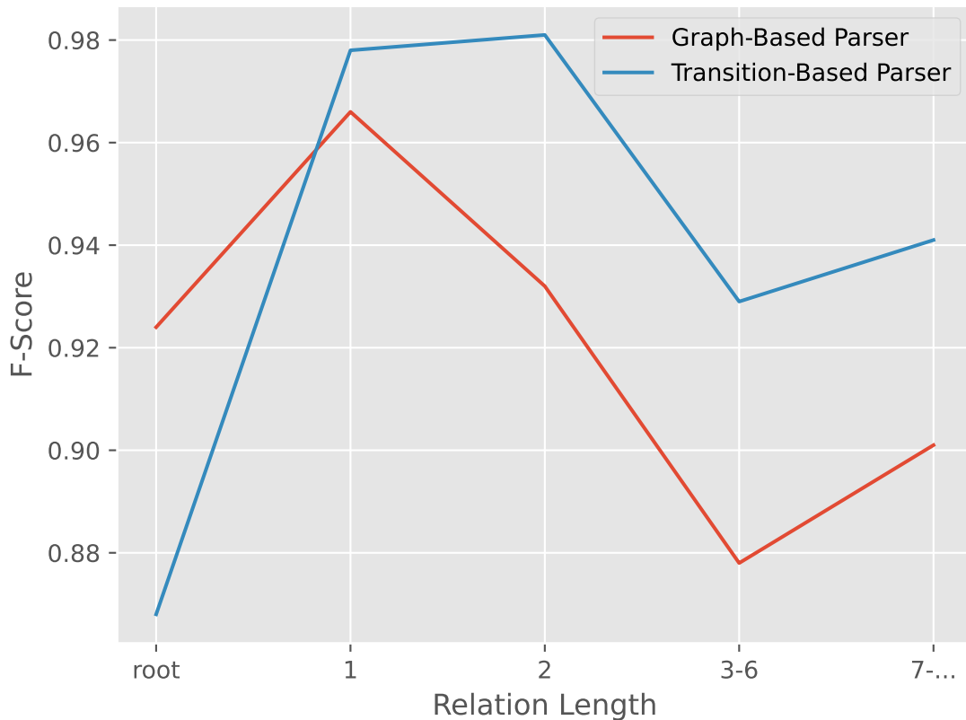
Relation Length vs F-Score
