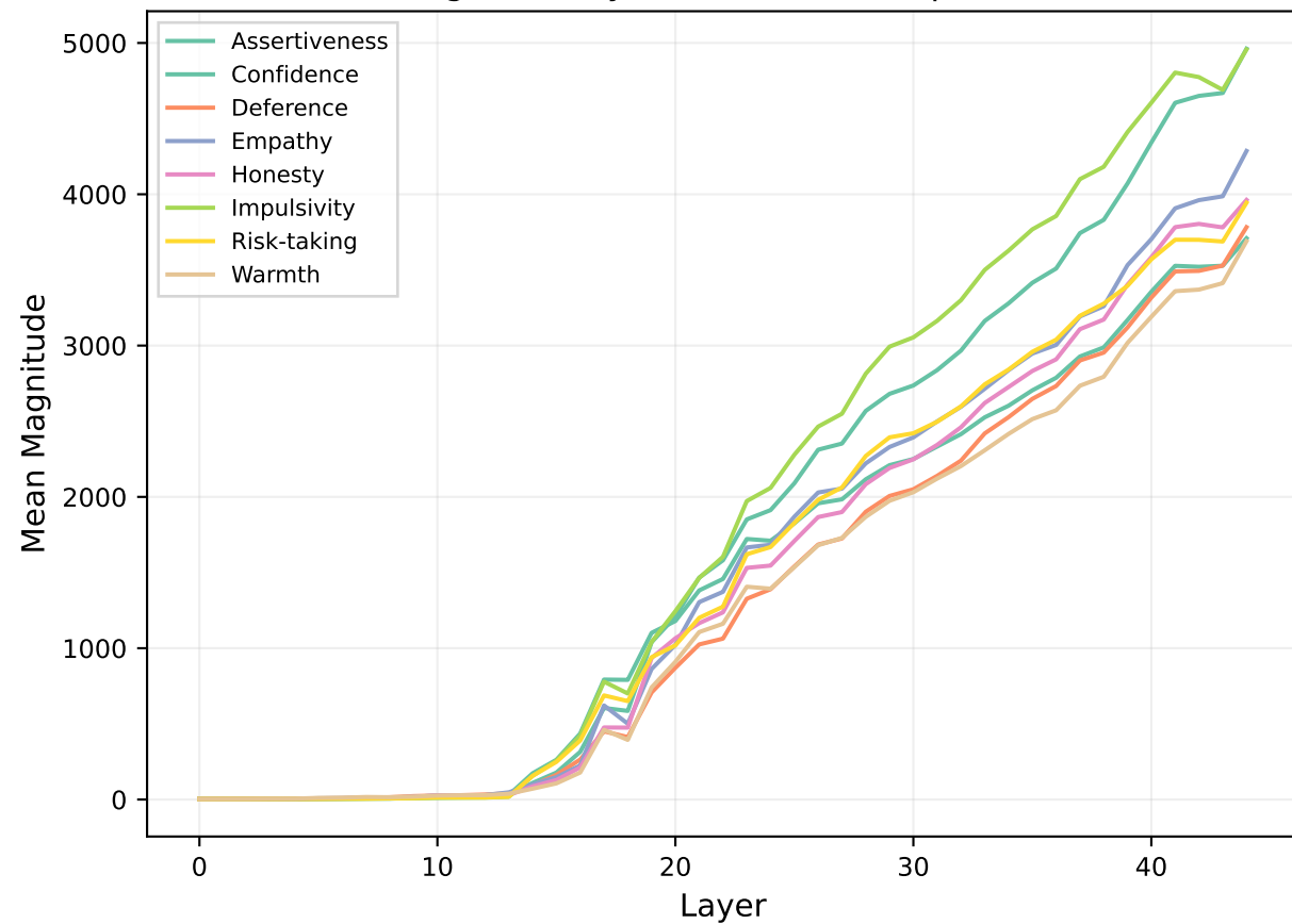
A) Magnitude by Trait (mean over personas)
