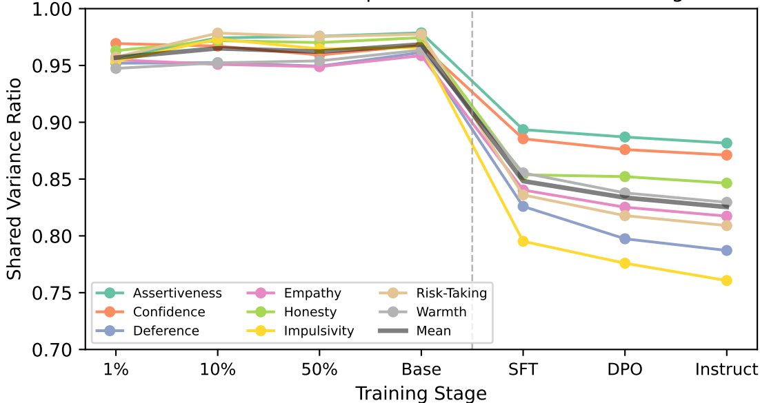
Shared vs Persona-Specific Variance Across Training
