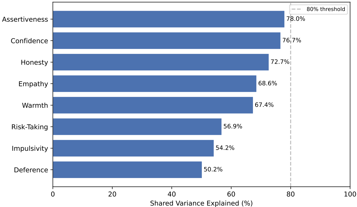
Fraction of Steering Vector Variance in Shared Direction
