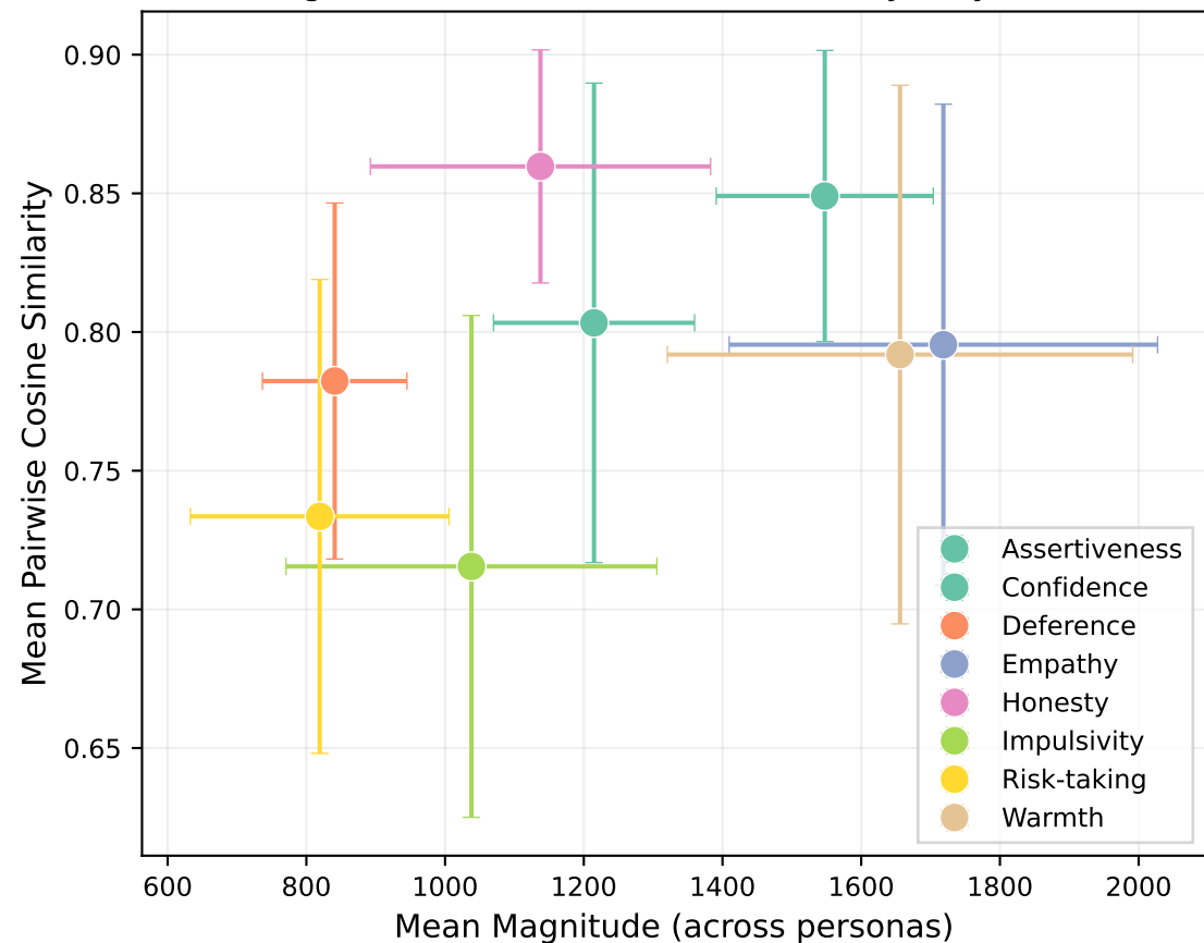
Magnitude vs Directional Consistency (Layer 25)
