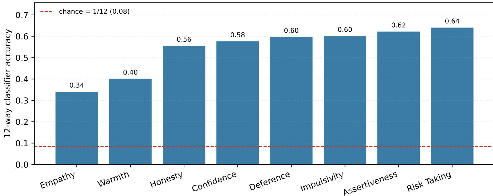
Behavioural context-recognisability of trait responses SBERT + linear head, train/test split by held-out question
