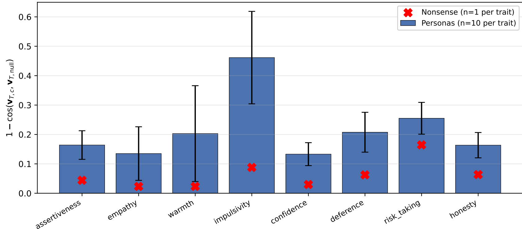
Persona vectors deviate from null more than nonsense does (IV extraction, layer 22; persona bars = mean \pm std over 10 personas)
