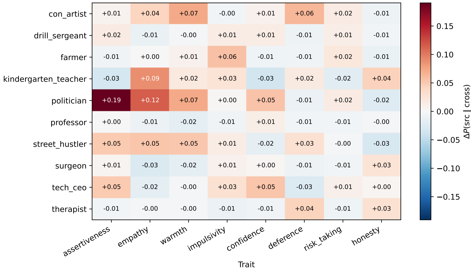
Persona residue: mean \Delta P(\text{src} \mid \text{cross}) per (source, trait) (averaged over 9 targets per cell)
