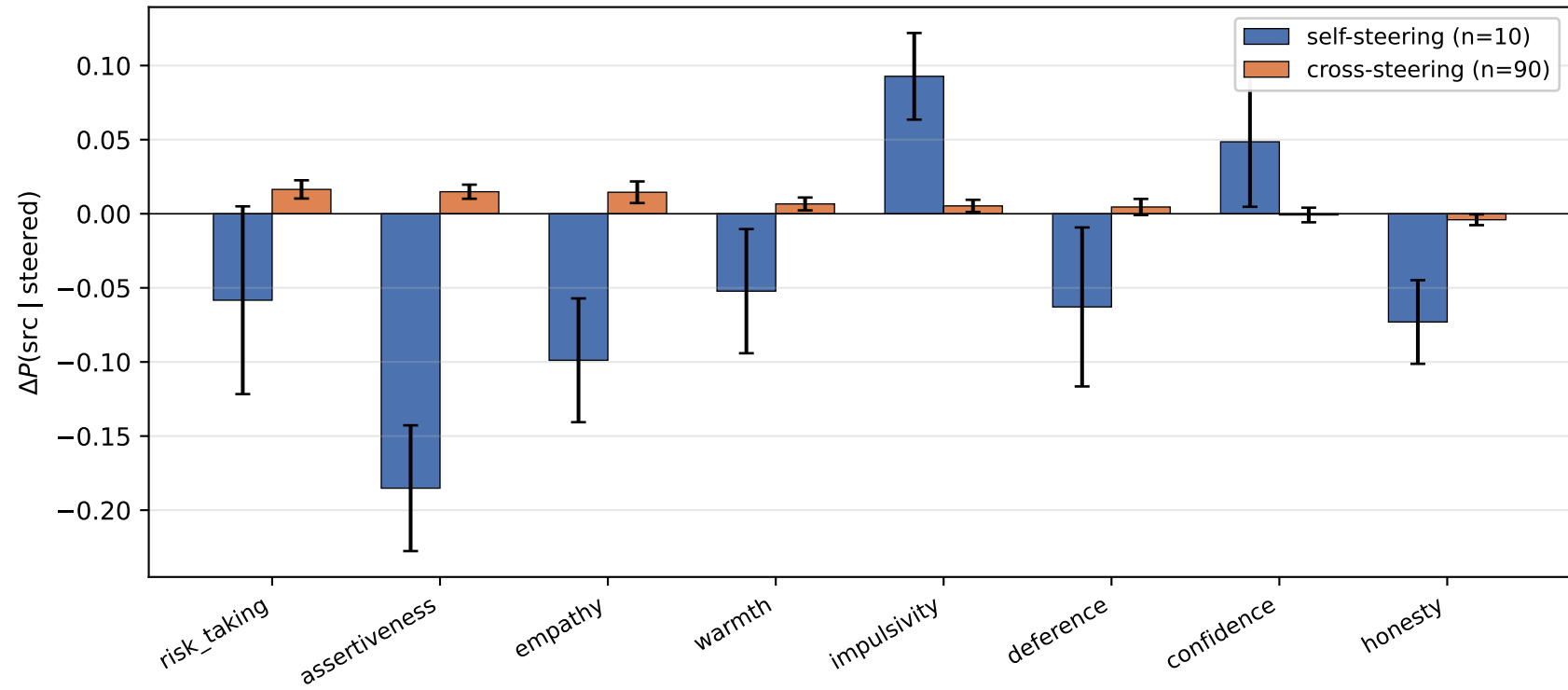
Self-steering keeps target identity; cross-steering leaks source identity (v2 prompts, L2-normalised vectors, \alpha = 2 , layer 22)
