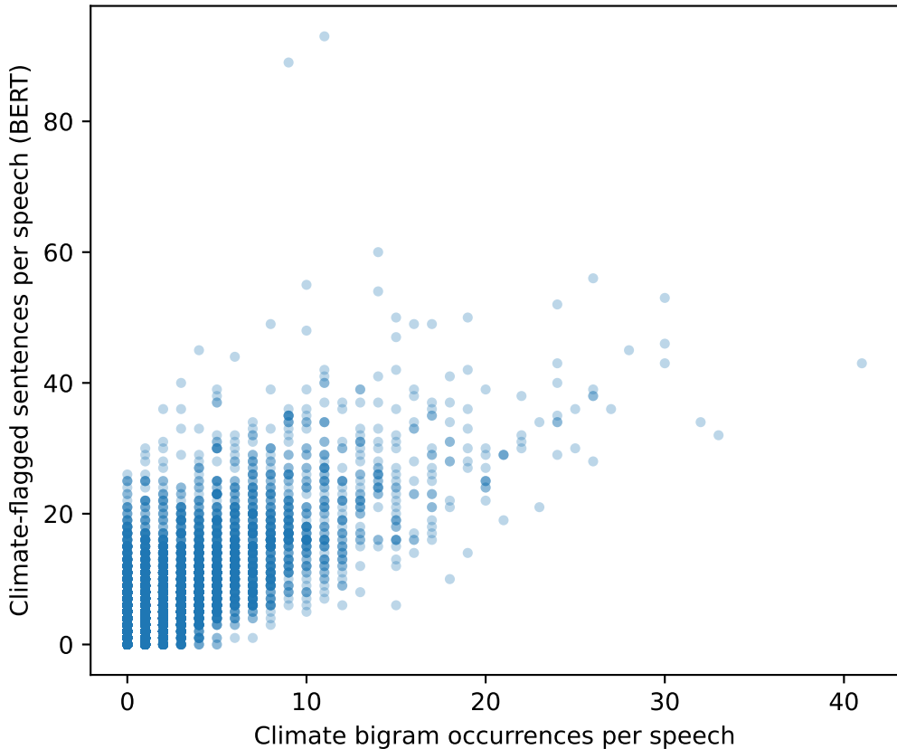
Speech-level agreement (Spearman \rho = 0.63 )
