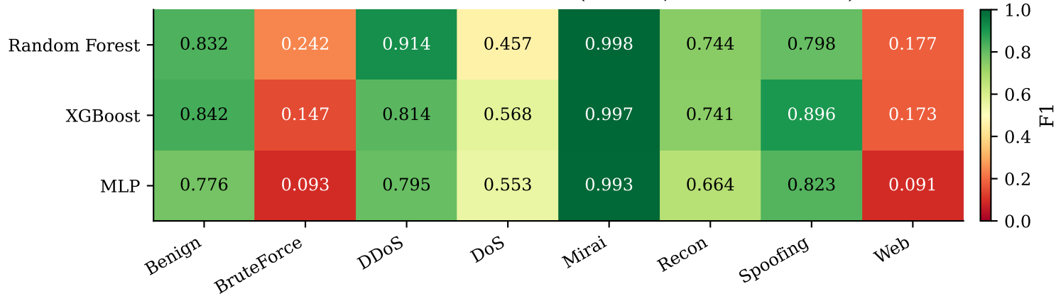
Per-class F1 across detectors (test set, mean of 5 seeds)
