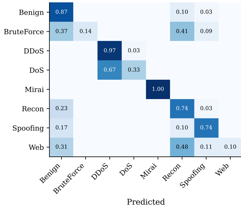
Random Forest
