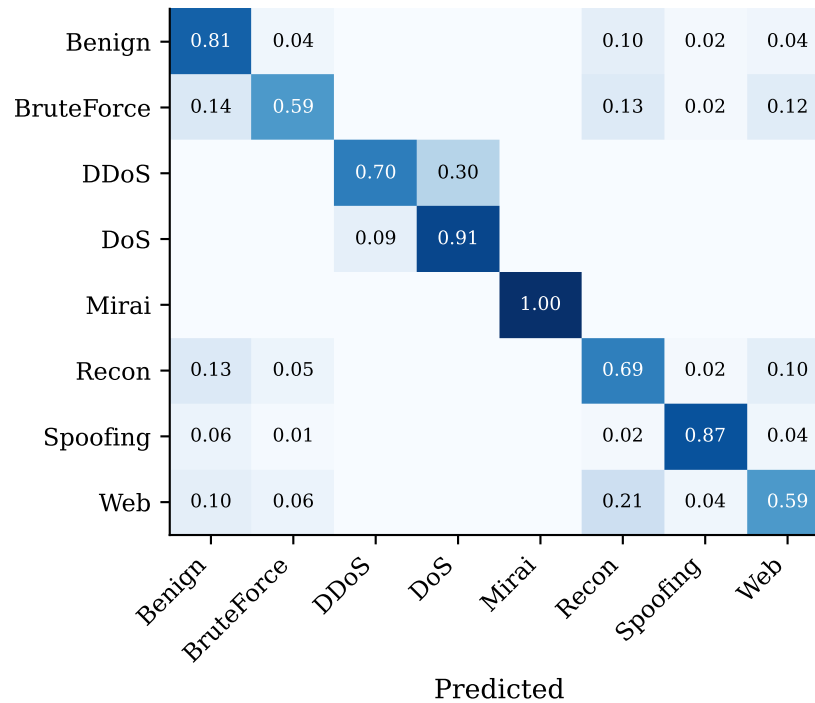
XGBoost
