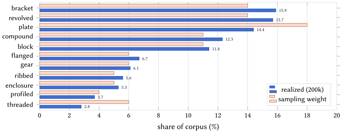
Figure 5. Realized family distribution on a 200k generation vs. the configured sampling weights. Realized shares drift below weight for low-diversity families (threaded, profiled) because dedup removes saturating repeats, and above weight where tier clamps add parts (bracket). All weights are tunable in configs/default.toml .
