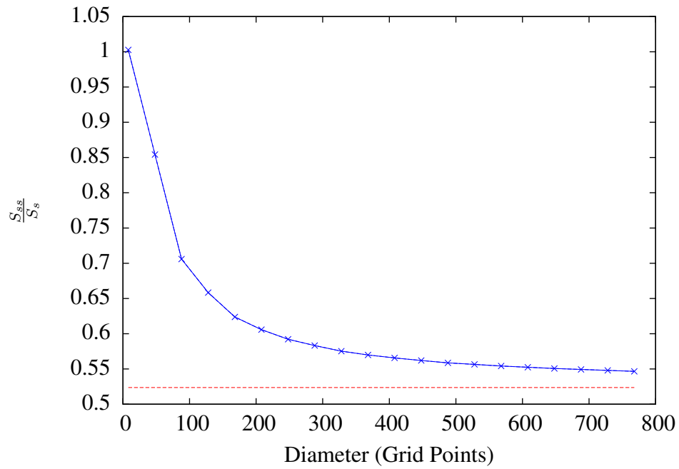
Figure 5.2: The fraction of memory used by the semi-structured approach with respect to the structured approach.
