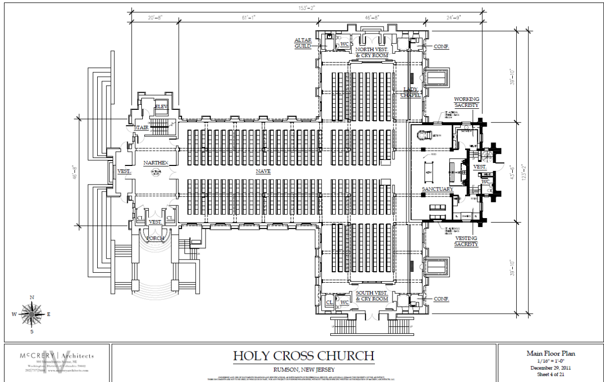
Figure 3.1: A diagram showing a schematic of a church building. Credit: McCrary Architects.
