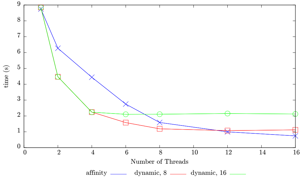
Figure 2: Graph showing execution time for loop 2 against number of threads for the affinity, dynamic, 8 and dynamic, 16 schedules.
