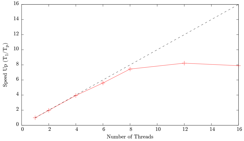
Figure 3: Speed Up for the dynamic 8 schedule
