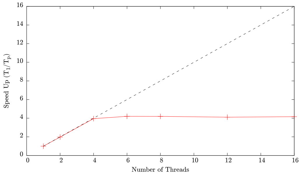
Figure 4: Speed Up for the dynamic 16 schedule
