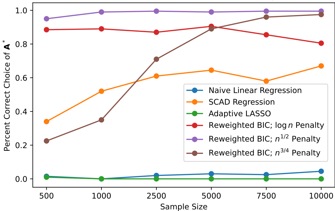
Simulation Results for the Backdoor Graph
