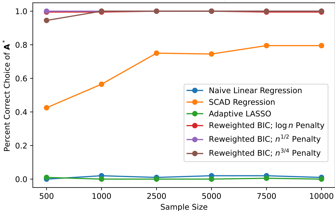
Simulation Results for the Backdoor Graph with Oracle Weights
