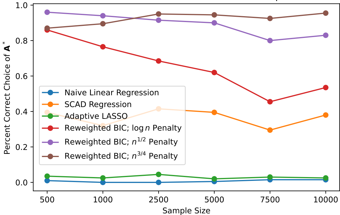
Simulation Results for the Frontdoor Graph
