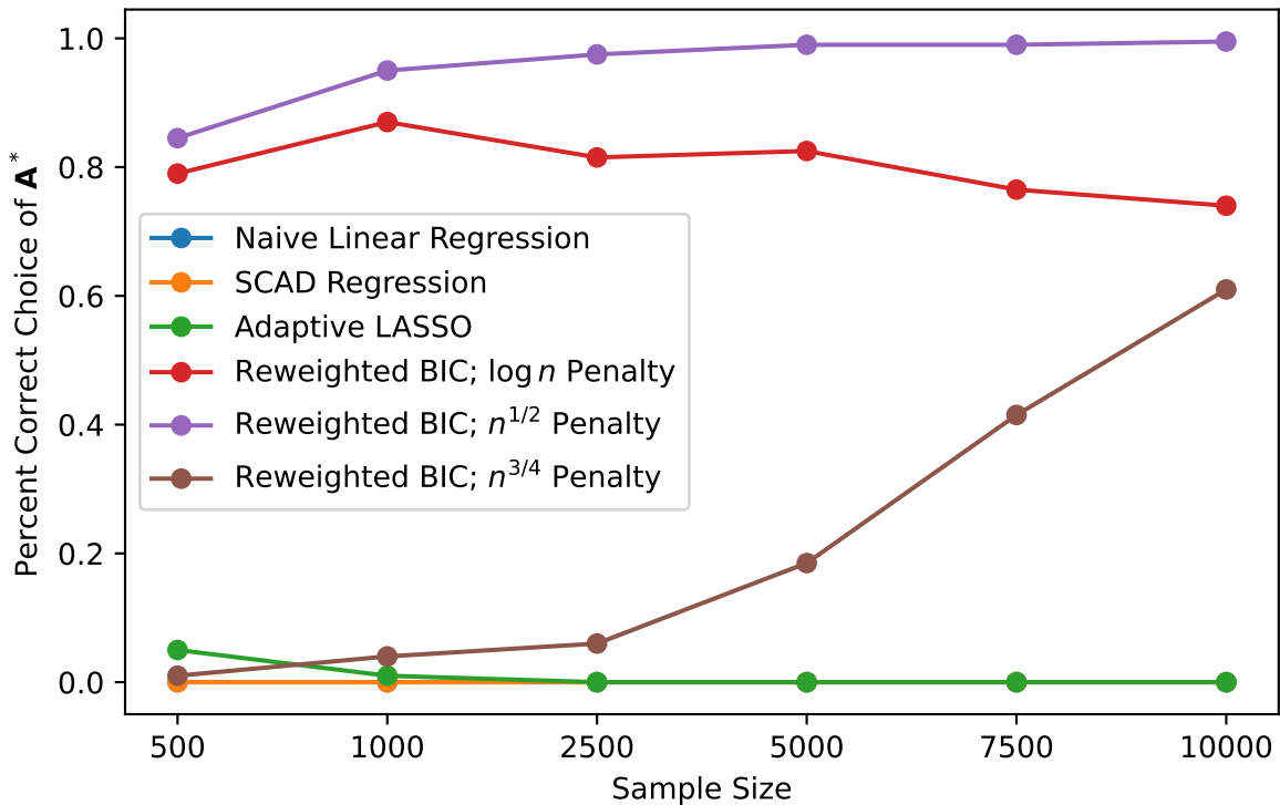
Simulation Results for the Frontdoor Graph
