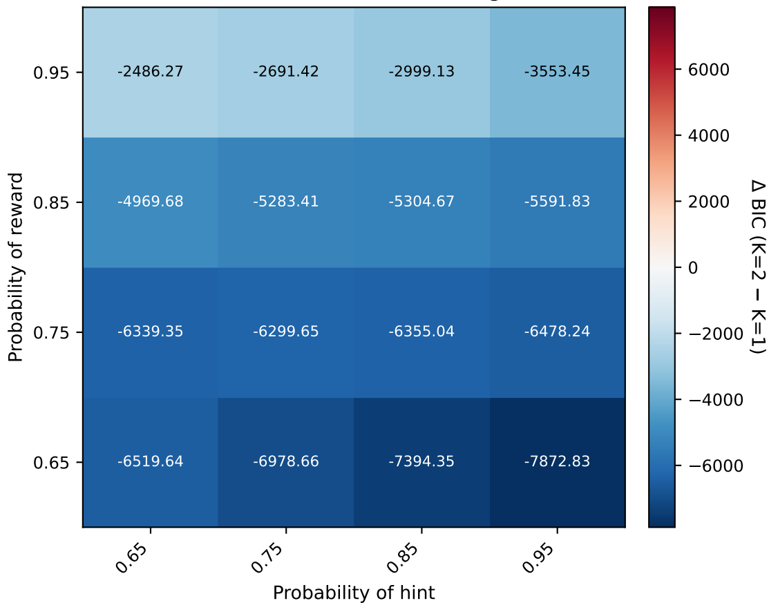
\Delta \text{BIC (K=2 - K=1)} — Averaged
