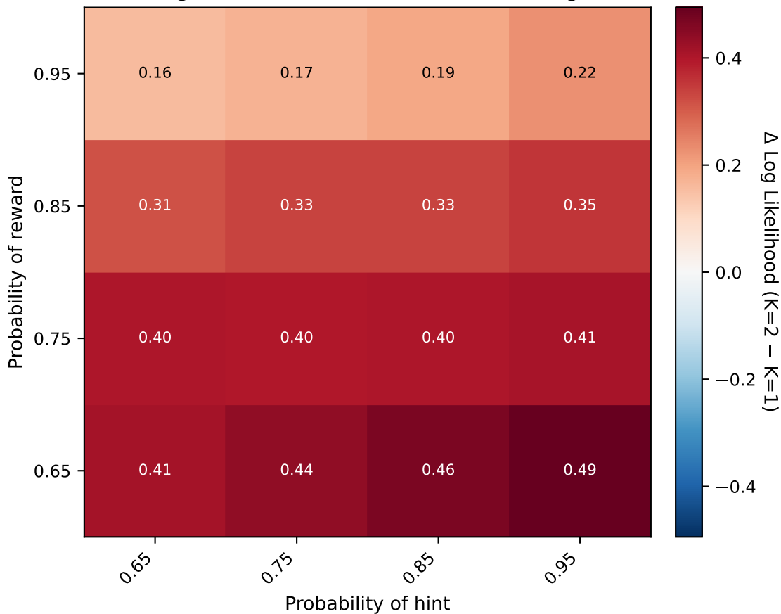
\Delta Log Likelihood (K=2 – K=1) — Averaged
