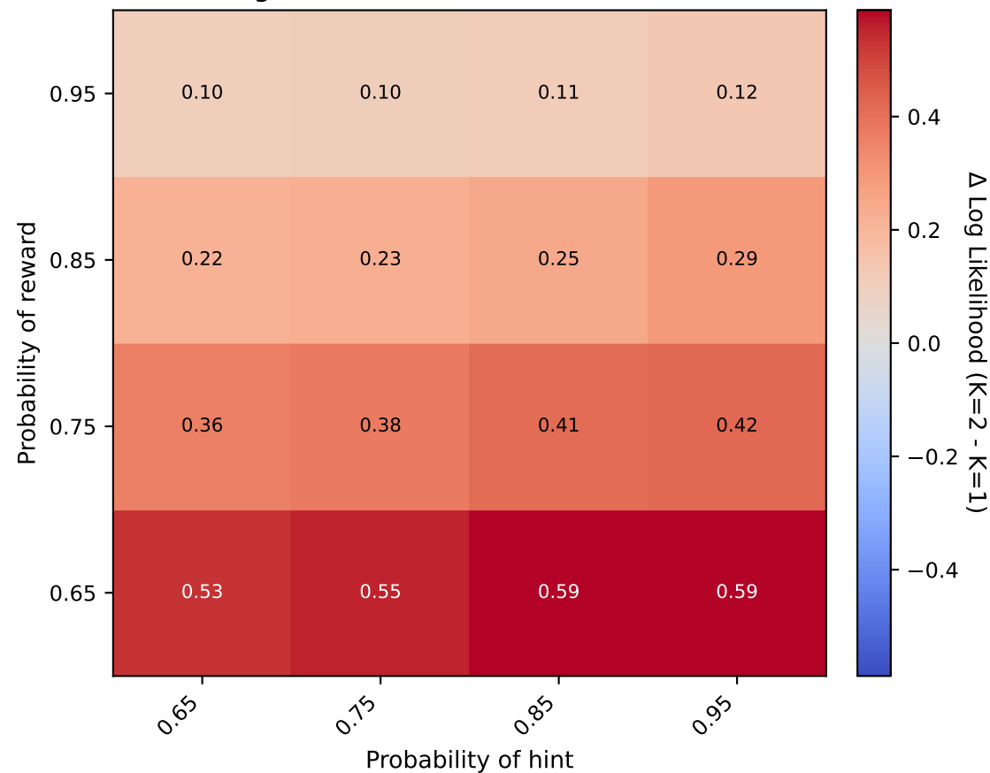
\Delta Log Likelihood (K=2 - K=1) — Case B
