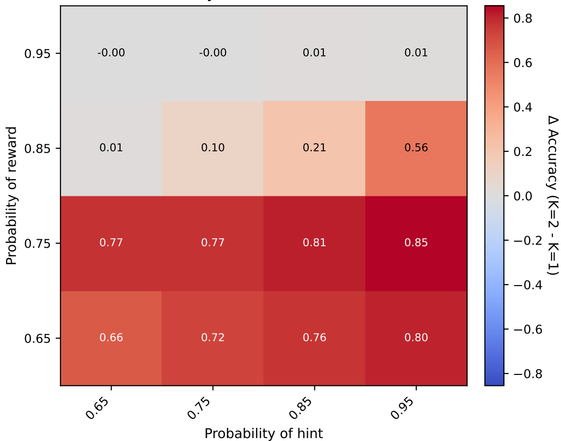
\Delta Accuracy (K=2 - K=1) — Case C
