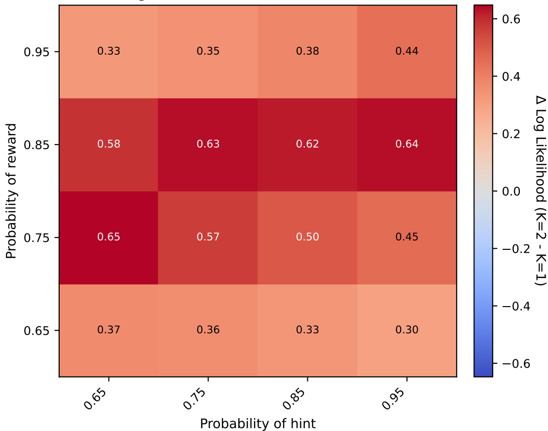
\Delta Log Likelihood (K=2 - K=1) — Case C
