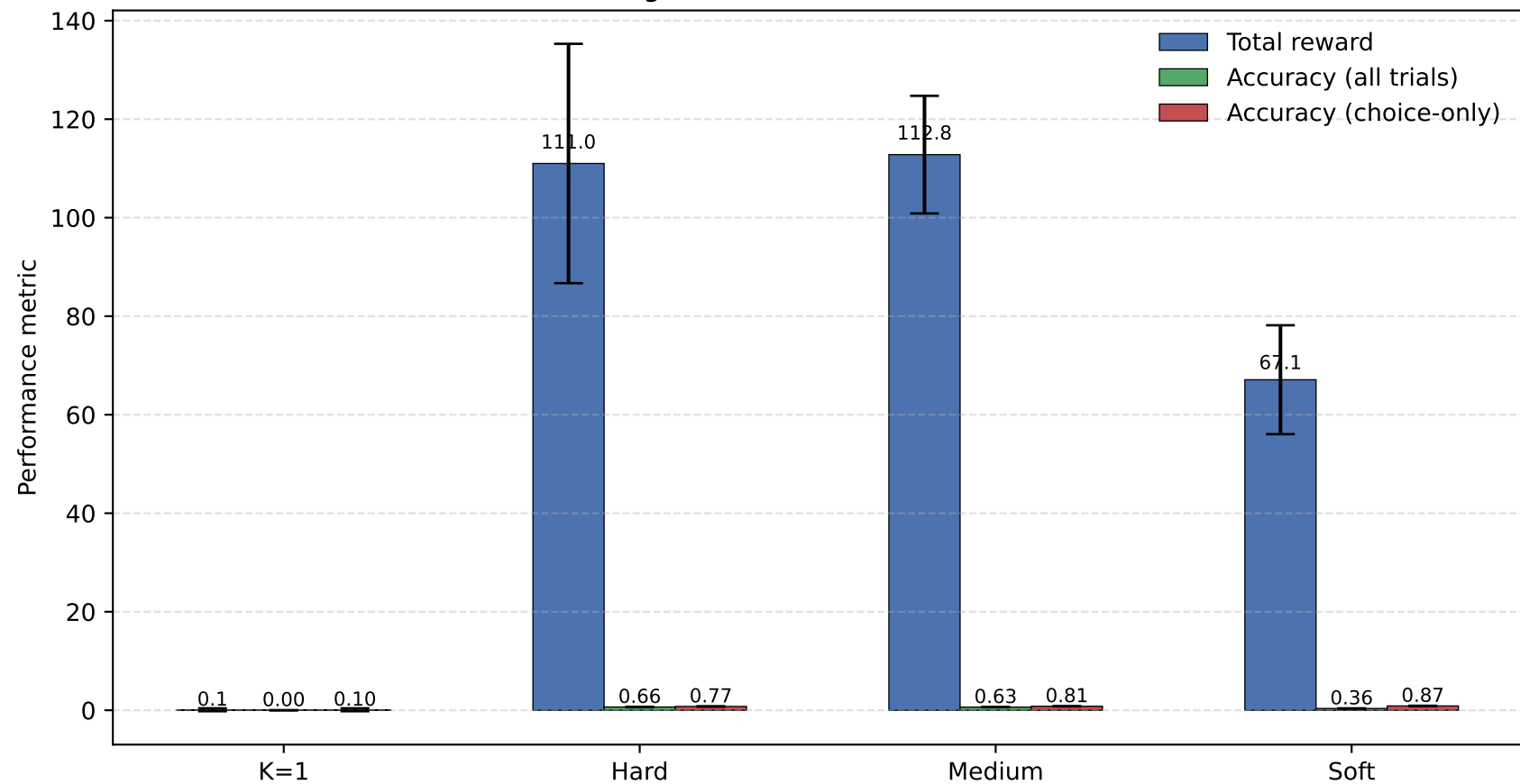
Ablation: Z-matrix mixing — Profile set C (P(reward)=0.65, P(hint)=0.65)
