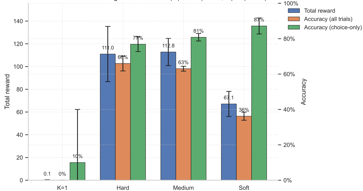
Ablation: Z-matrix mixing — Profile set C ( P(\text{reward})=0.65 , P(\text{hint})=0.65 )
