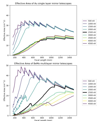
Fig. 9: Effective area of Wolter-I mirrors across a range of focal lengths. Boosts in area are a result of nesting additional shells at longer focal lengths when mirrors are more horizontal. Energy bands show how lower energies are maximally reflected by larger geometric area found with higher incidence angles and sufficient reflectivity.
