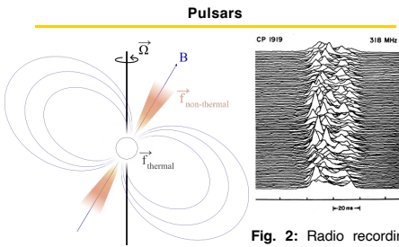
Fig. 2: Radio recording of Pulsar CP 1919 (PSR B1919+21) [4] showing variation of individual pulse profiles, but steady phase.
