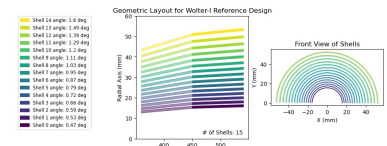
Fig. 8: Cross sections of a Wolter-I telescope design with parabolic and hyperbolic stages, maximally nested shells, and parameters described in the Model Parameter table. The figure shows the specific case for 450 mm Focal Length, which includes fifteen complete shells.
