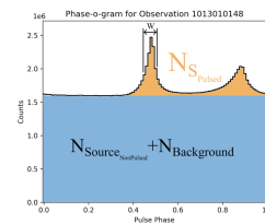
Fig. 5: A histogram of counts versus pulse phase for Observation ID 1013010148 of the Crab Pulsar, PSR B0531+21. The non-pulsed source emission and background emission are indistinguishable and combine to fill the static blue region of the plot. The Pulsed source emission forms the dynamic orange region at the top of the plot. The pulse width, W , is annotated. Note that counts on the Y-axis are scaled by one million.
