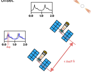
Fig. 4: Illustration of pulsar-informed navigation. Two observations of a distant pulsar are made at different locations, introducing a measurable phase shift, \Delta\phi , between the peaks of the measured pulses. The physical distance along the direction to the pulsar, \Delta r , is directly related to this phase shift by the relation c\Delta\phi/f , where c is the speed of light and f is the pulsar rotation frequency.
