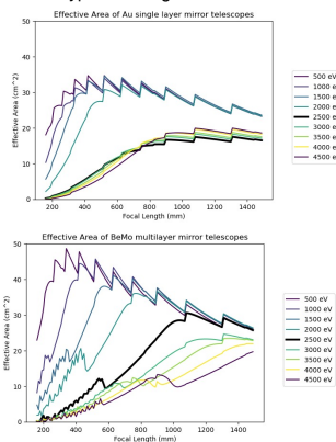
Fig. 9: Effective area of Wolter-I mirrors across a range of focal lengths. Boosts in area are a result of nesting additional shells at longer focal lengths when mirrors are more horizontal. Energy bands show how lower energies are maximally reflected by larger geometric area found with higher incidence angles and sufficient reflectivity.
