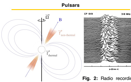
Fig. 2: Radio recording of Pulsar CP 1919 (PSR B1919+21) [4] showing variation of individual pulse profiles, but steady phase.
