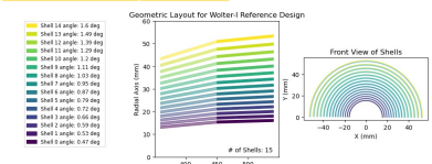
Fig. 8: Cross sections of a Wolter-I telescope design with parabolic and hyperbolic stages, maximally nested shells, and parameters in the following table, with parameters described in the Model Parameter table for 450 mm Focal Length. Includes fifteen complete shells, each with parabolic and hyperbolic segments.
