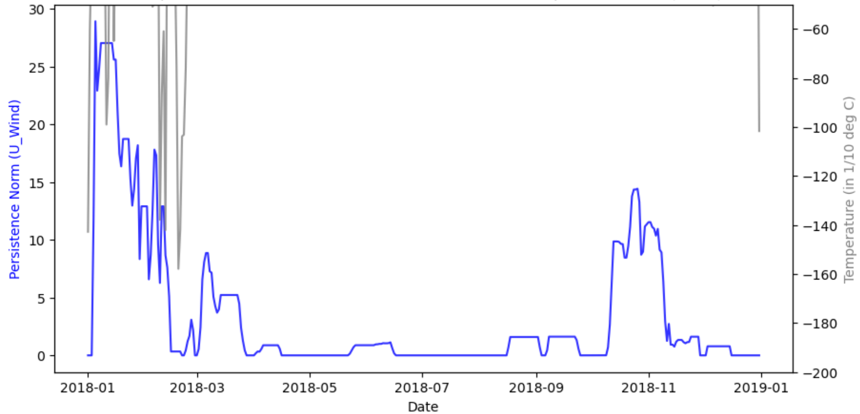
Comparison of Polar Wind Persistence Norms and Temperature Data (2018)
