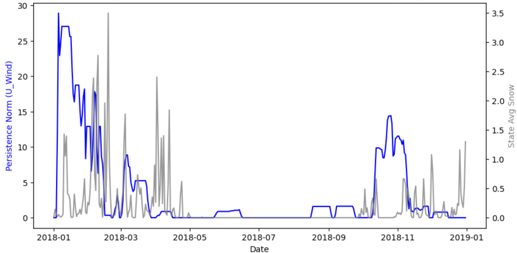
Comparison of Polar Wind Persistence Norms and Snow Data (2018)
