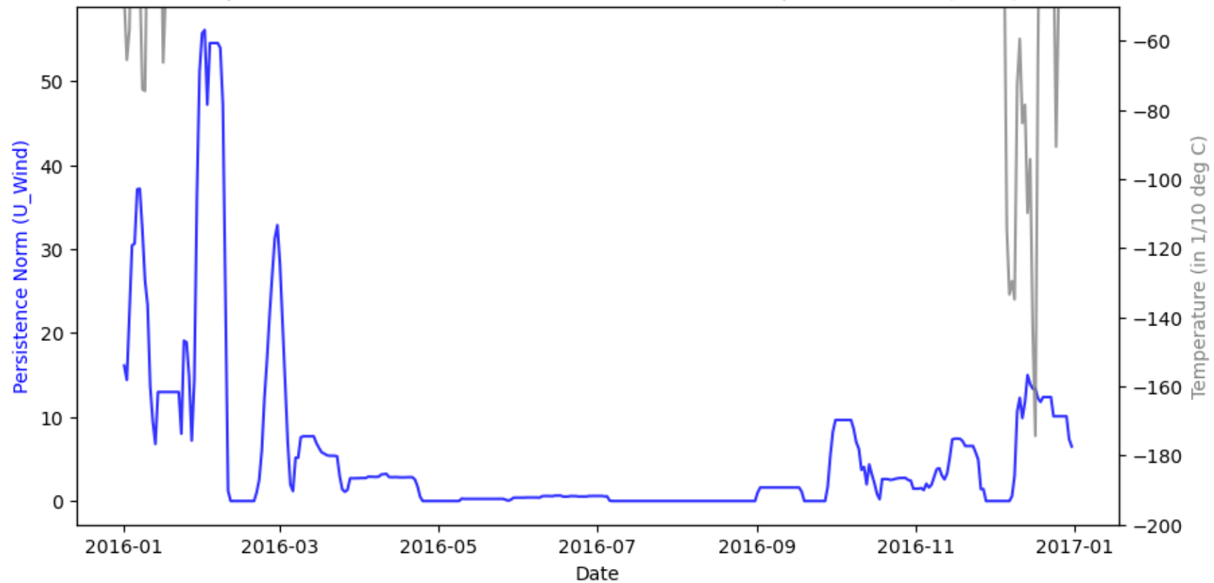
Comparison of Polar Wind Persistence Norms and Temperature Data (2016)
