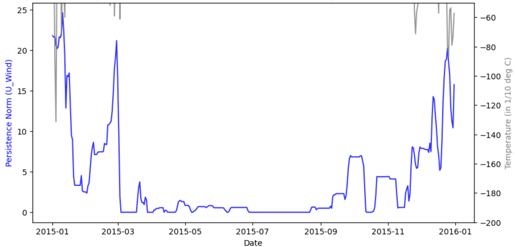
Comparison of Polar Wind Persistence Norms and Temperature Data (2015)
