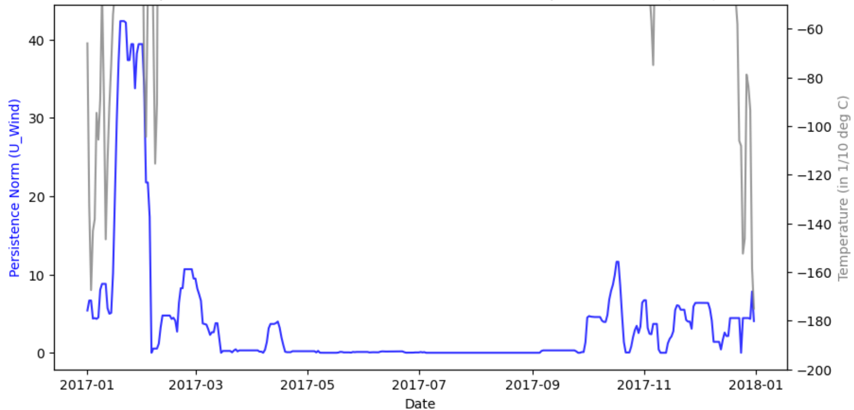
Comparison of Polar Wind Persistence Norms and Temperature Data (2017)
