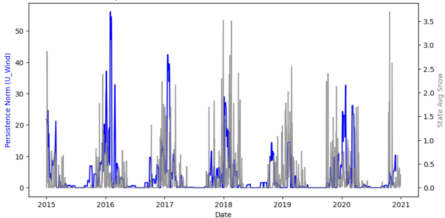
Comparison of Polar Wind Persistence Norms and Snow Data
