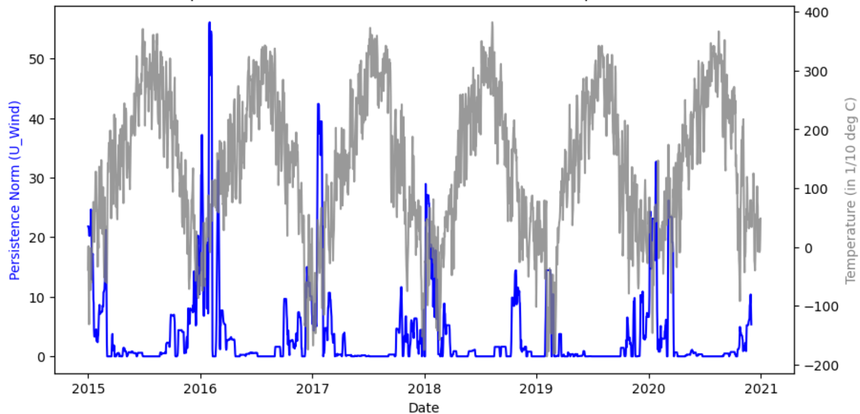
Comparison of Polar Wind Persistence Norms and Temperature Data
