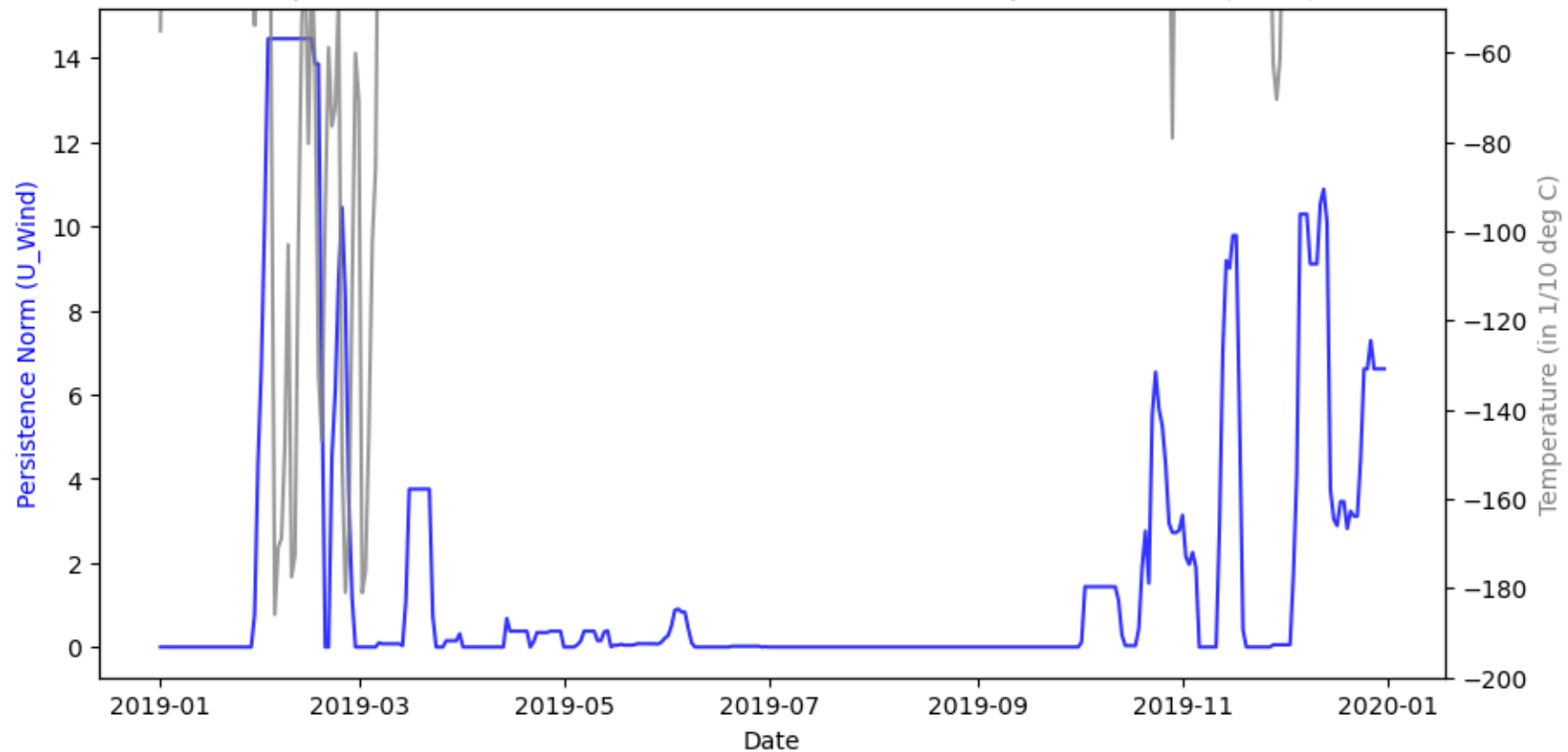
Comparison of Polar Wind Persistence Norms and Temperature Data (2019)
