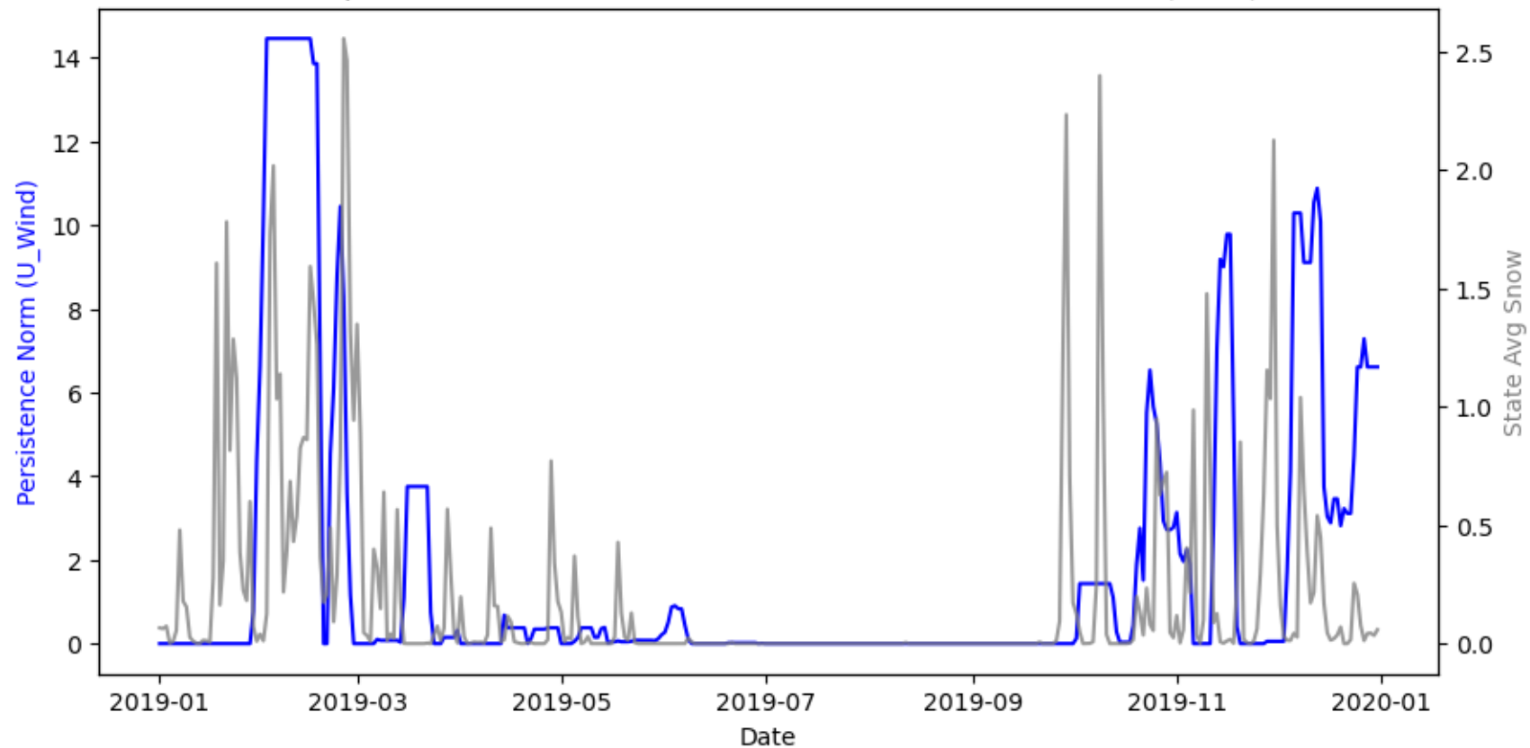
Comparison of Polar Wind Persistence Norms and Snow Data (2019)
