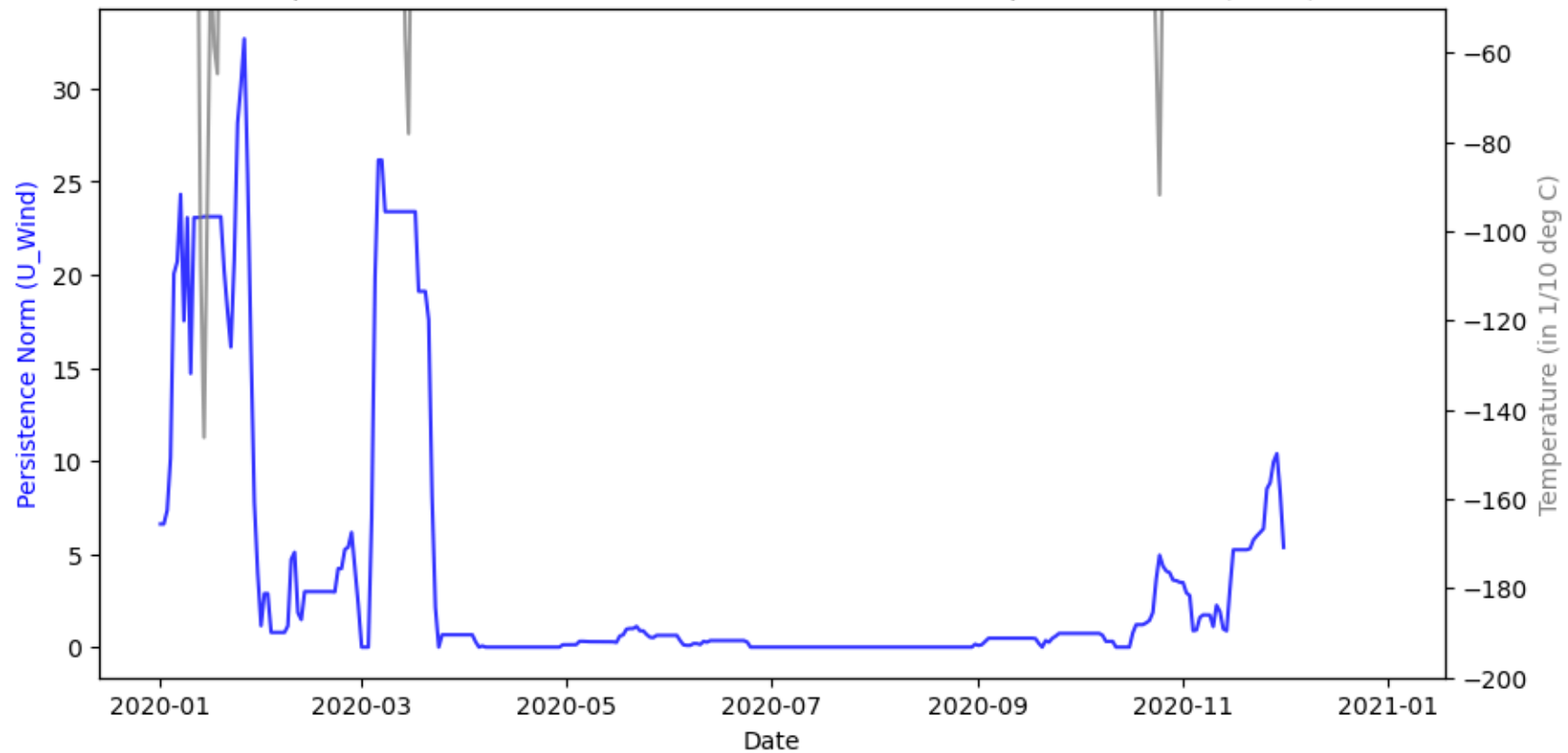
Comparison of Polar Wind Persistence Norms and Temperature Data (2020)
