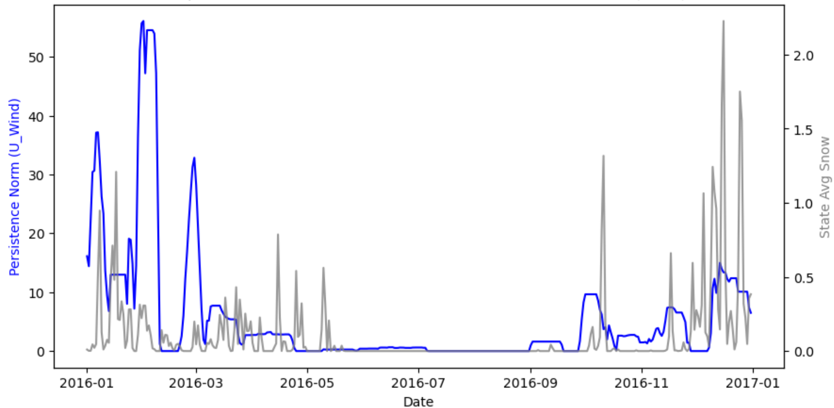
Comparison of Polar Wind Persistence Norms and Snow Data (2016)
