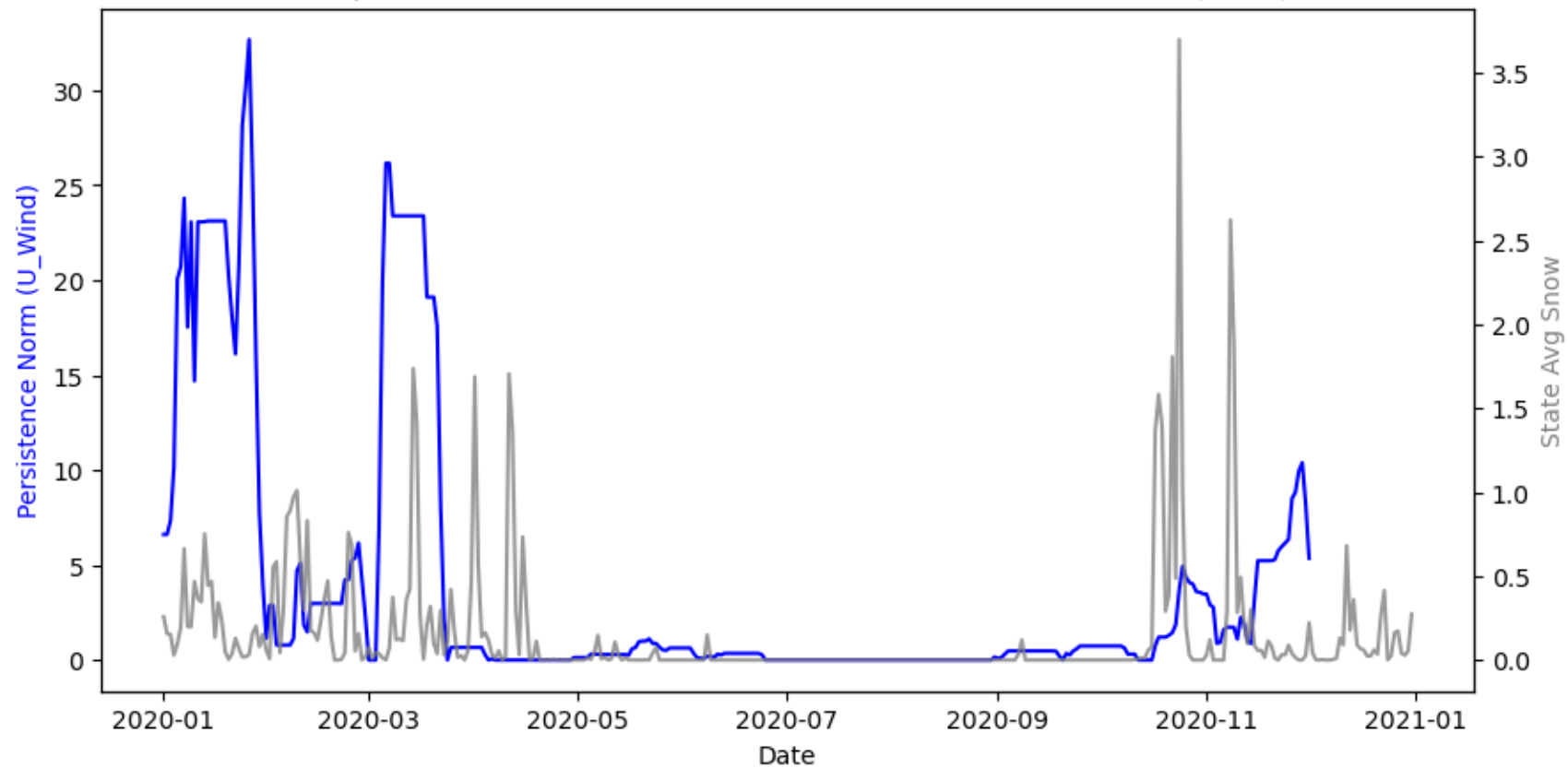
Comparison of Polar Wind Persistence Norms and Snow Data (2020)
