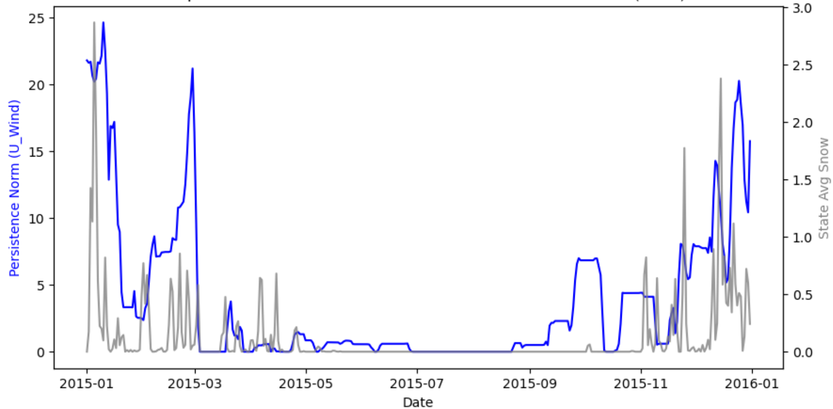
Comparison of Polar Wind Persistence Norms and Snow Data (2015)
