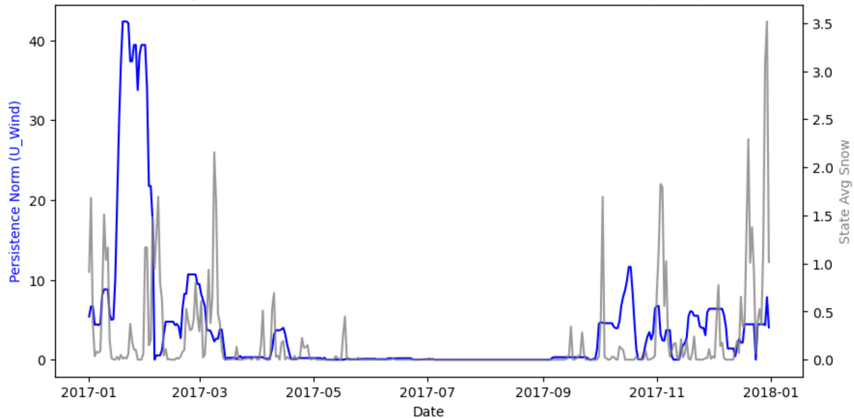
Comparison of Polar Wind Persistence Norms and Snow Data (2017)
