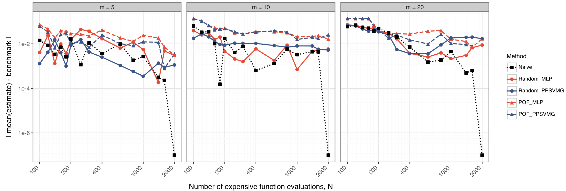
SIR: absolute bias against N=2000 MC benchmark
