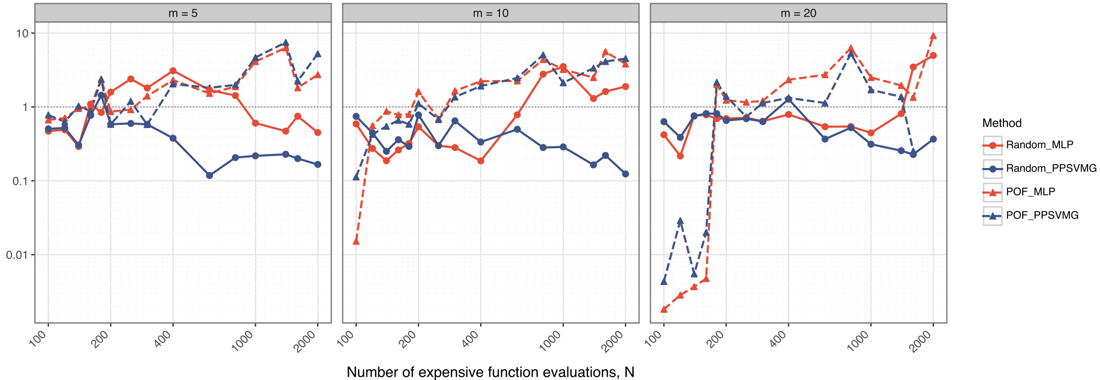
SIR: variance ratio ( < 1 = better than naive)
