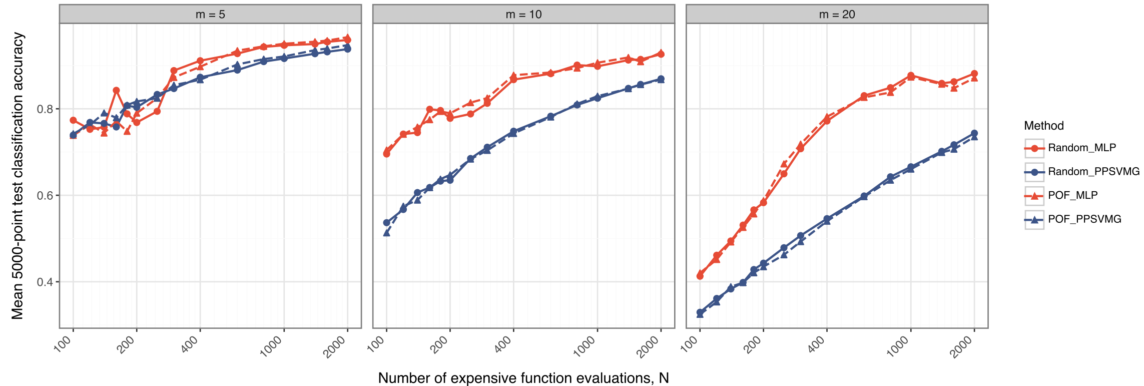
brusselator: classifier accuracy on held-out test set
