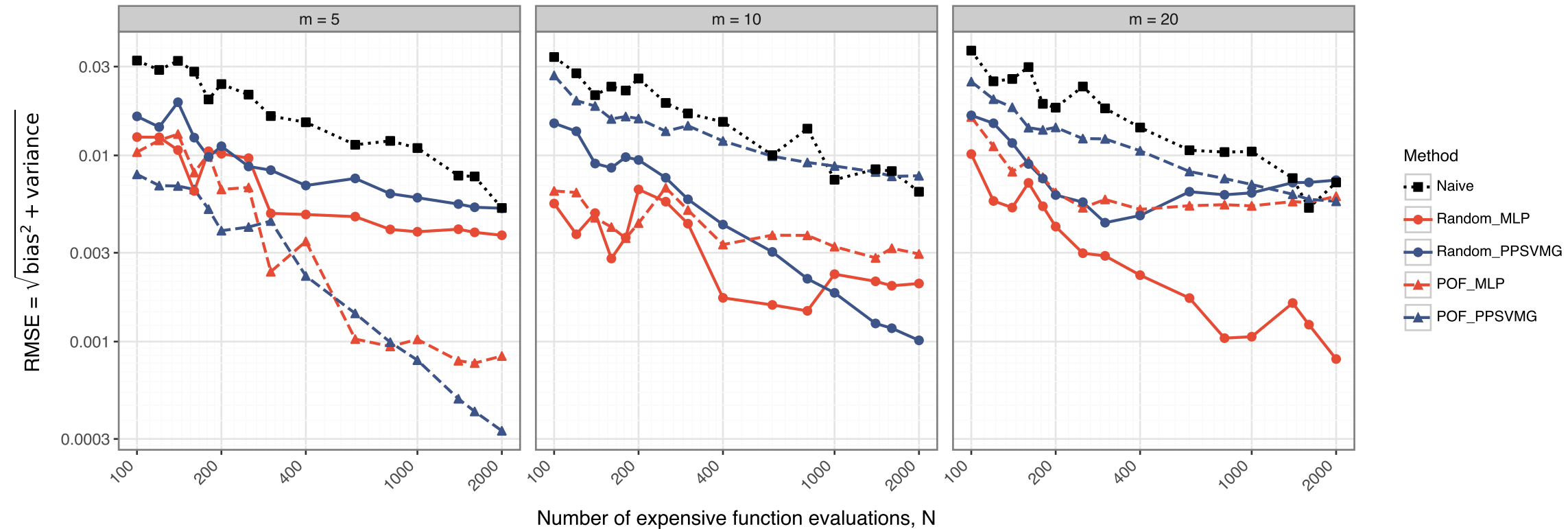
brusselator: root-mean-squared error
