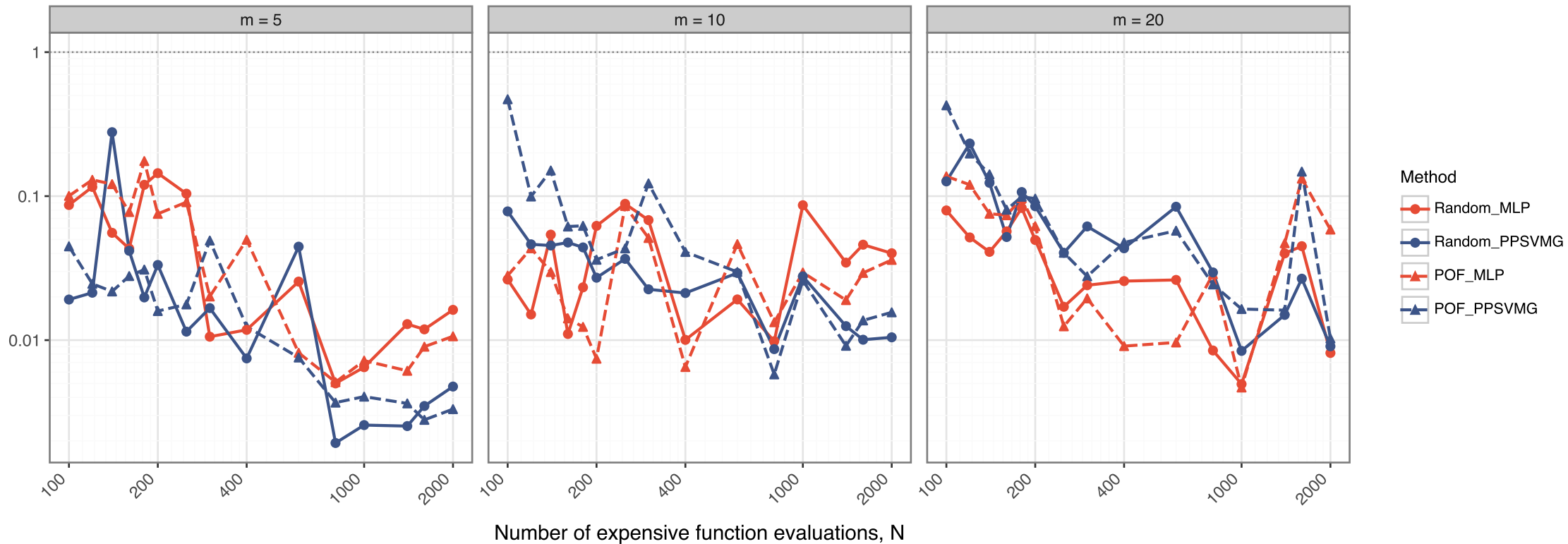
brusselator: variance ratio ( < 1 = better than naive)
