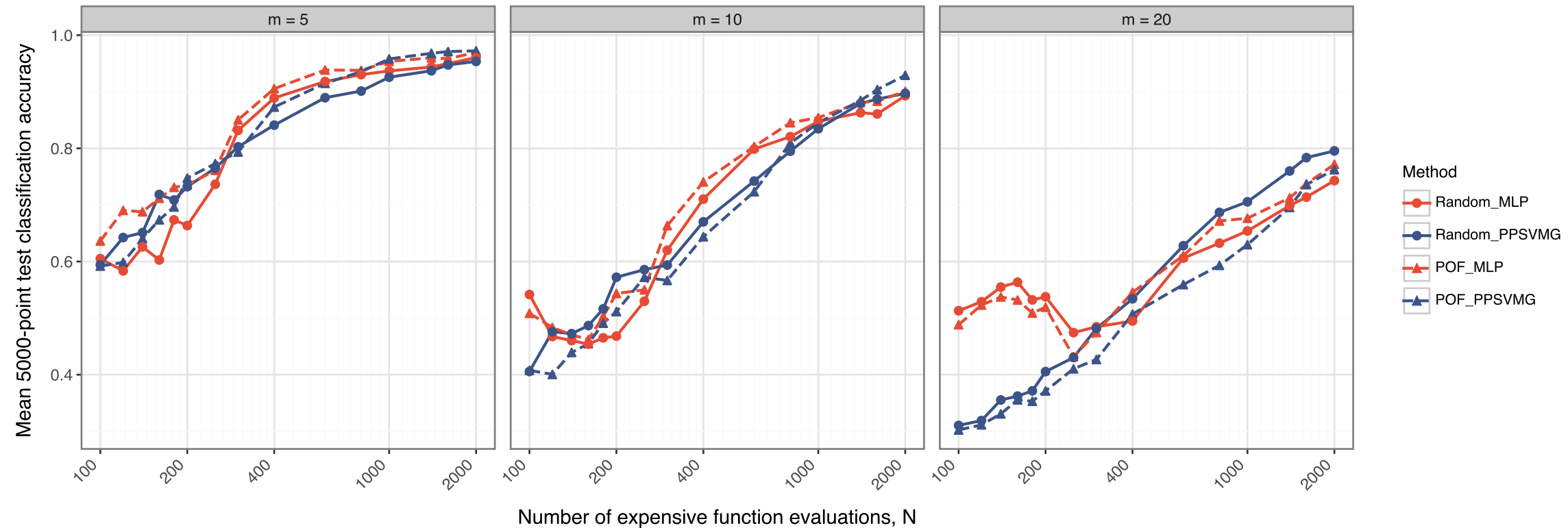
function2: classifier accuracy on held-out test set
