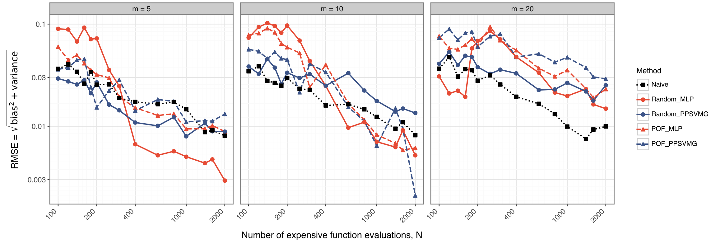
function2: root-mean-squared error
